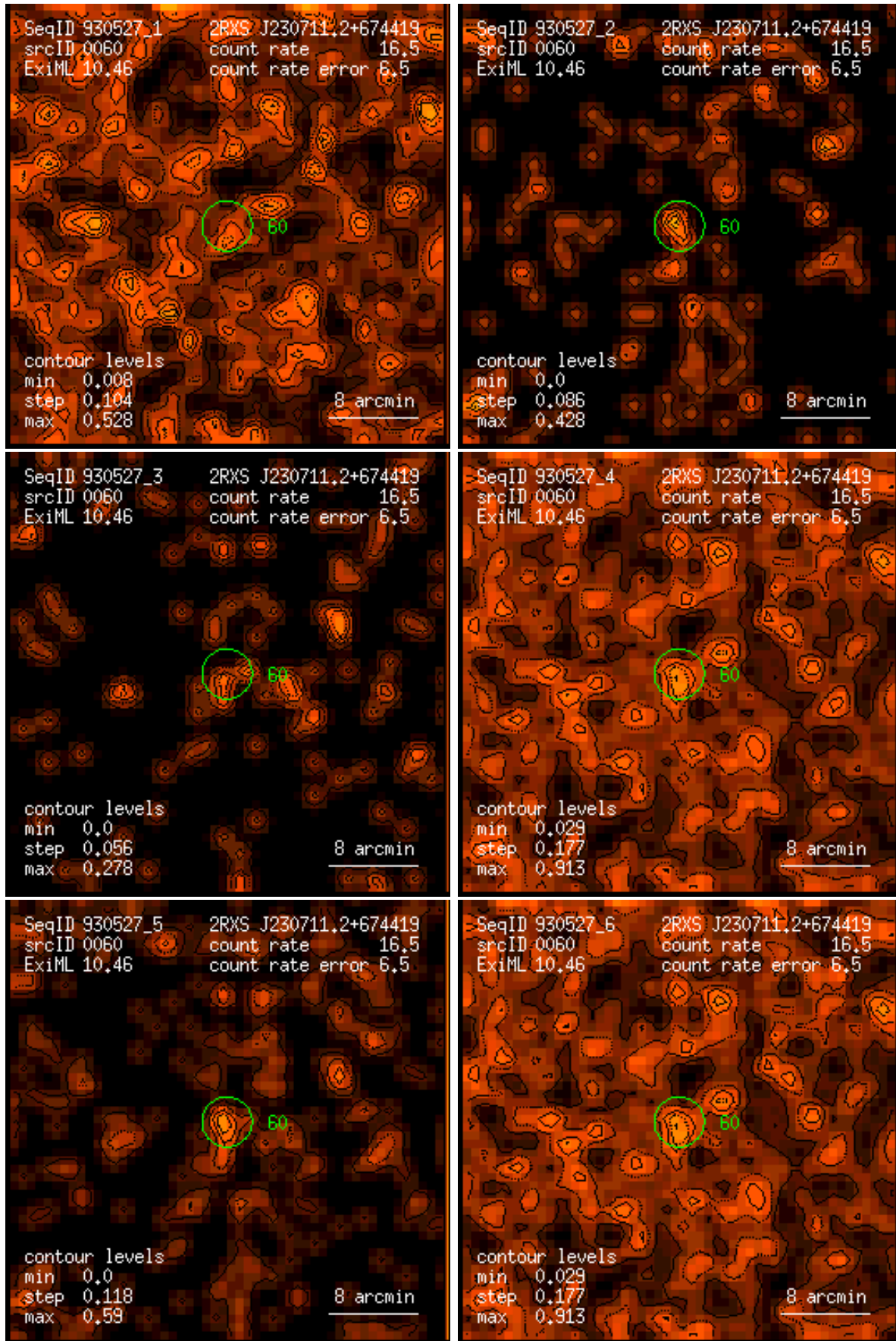
Figure 60: RASS 930527: detection 0060: band rate images, Gaussian filter: (1) PSPC channels 11 – 41, (2) 52 – 90, (3) 91 – 201, (4) 11 – 235, (5) 52 – 201, (6) 11 – 201. Broad band rates in counts/ks. Band rate contour levels in counts/ks/arcmin 2 .
