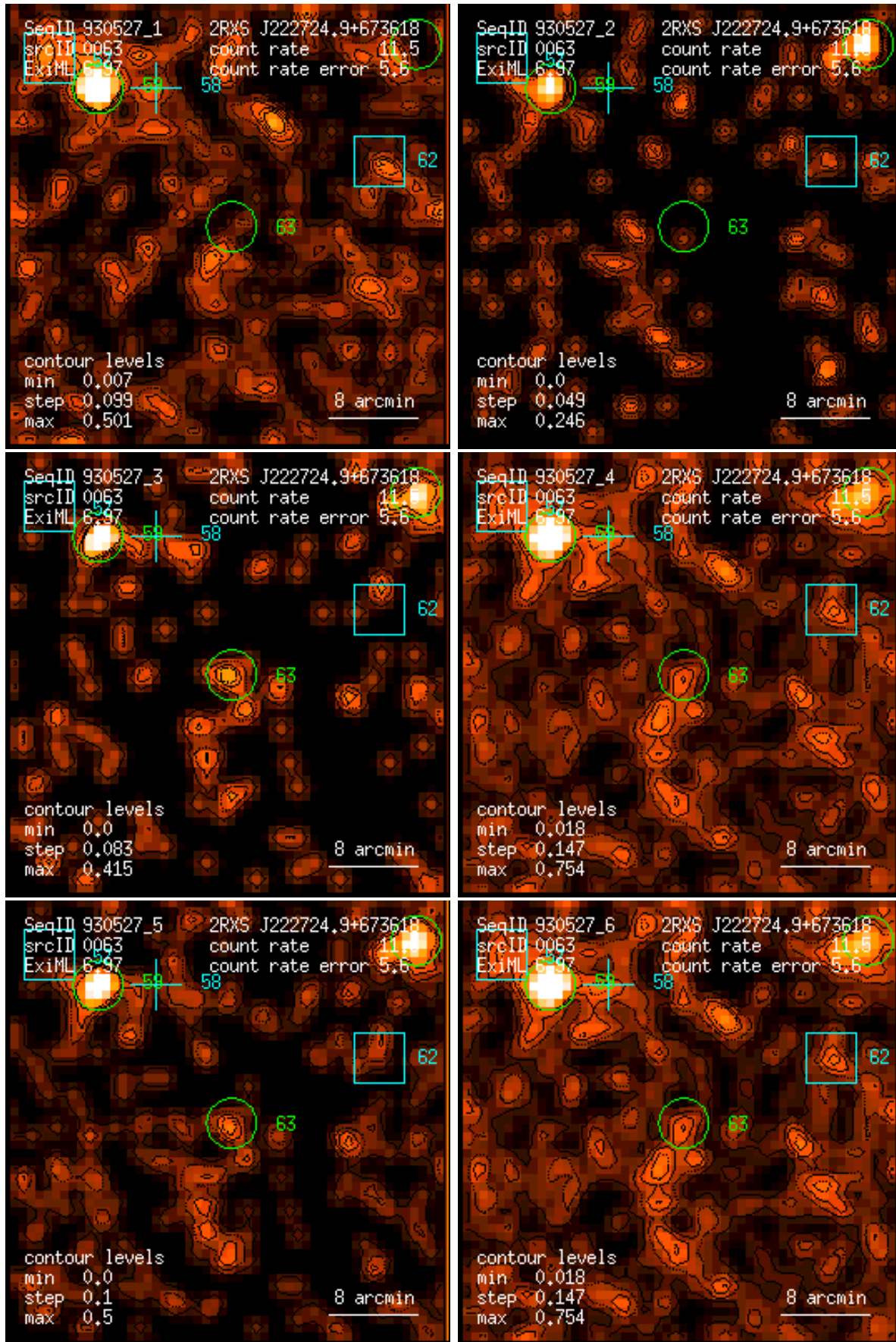
Figure 63: RASS 930527: detection 0063: band rate images, Gaussian filter: (1) PSPC channels 11 – 41, (2) 52 – 90, (3) 91 – 201, (4) 11 – 235, (5) 52 – 201, (6) 11 – 201. Broad band rates in counts/ks. Band rate contour levels in counts/ks/arcmin 2 .
