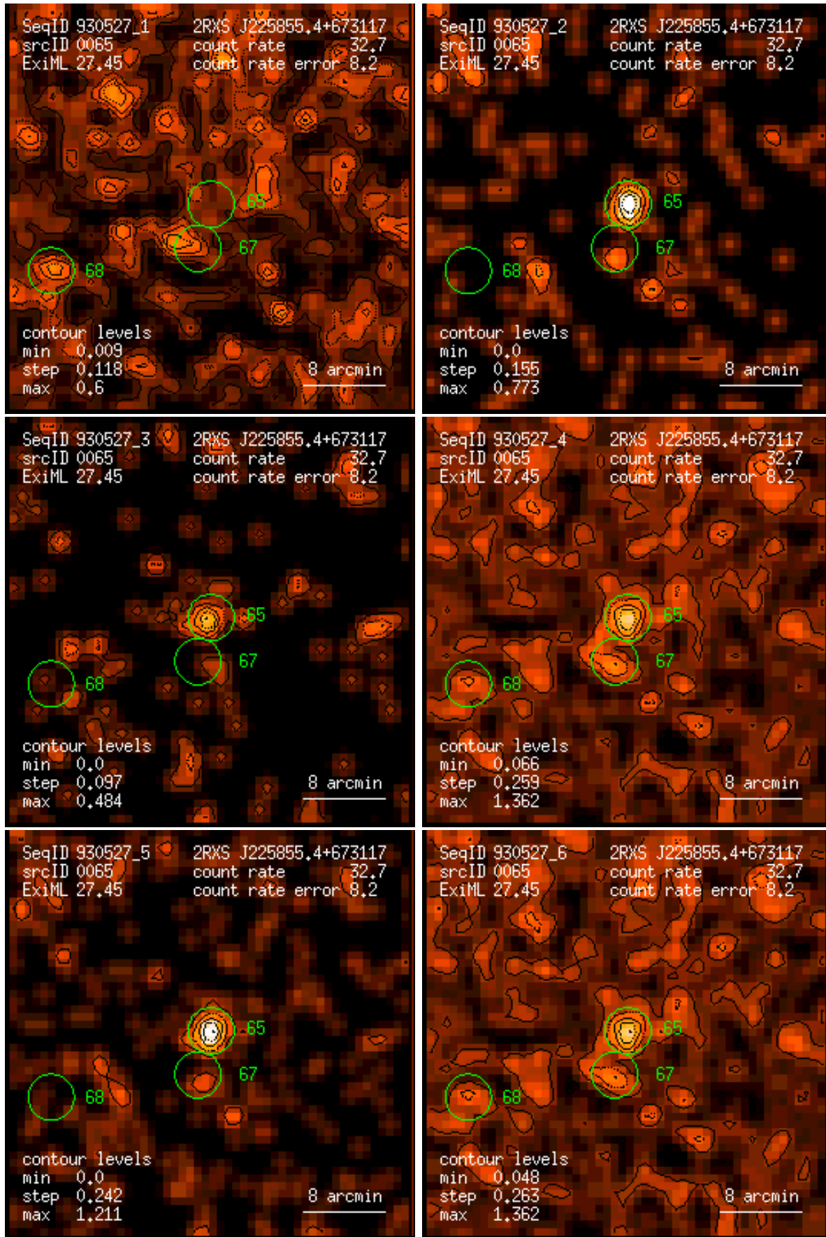
Figure 65: RASS 930527: detection 0065: band rate images, Gaussian filter: (1) PSPC channels 11 – 41, (2) 52 – 90, (3) 91 – 201, (4) 11 – 235, (5) 52 – 201, (6) 11 – 201. Broad band rates in counts/ks. Band rate contour levels in counts/ks/arcmin 2 .
