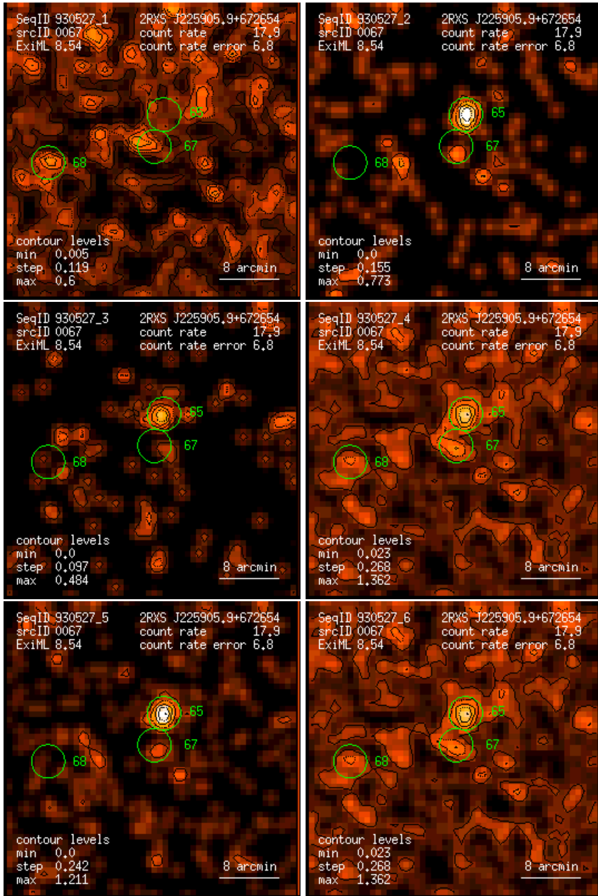
Figure 67: RASS 930527: detection 0067: band rate images, Gaussian filter: (1) PSPC channels 11 – 41, (2) 52 – 90, (3) 91 – 201, (4) 11 – 235, (5) 52 – 201, (6) 11 – 201. Broad band rates in counts/ks. Band rate contour levels in counts/ks/arcmin 2 .
