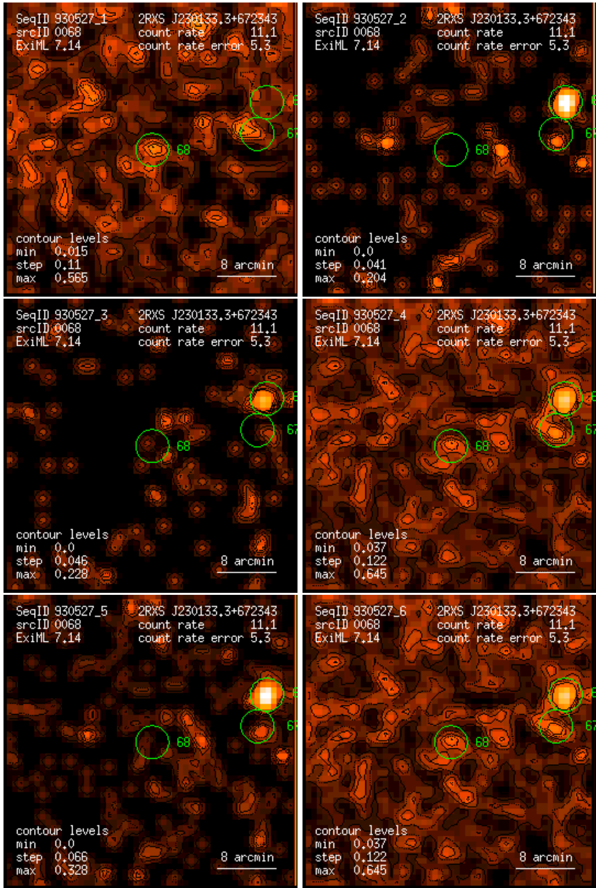
Figure 68: RASS 930527: detection 0068: band rate images, Gaussian filter: (1) PSPC channels 11 – 41, (2) 52 – 90, (3) 91 – 201, (4) 11 – 235, (5) 52 – 201, (6) 11 – 201. Broad band rates in counts/ks. Band rate contour levels in counts/ks/arcmin 2 .
