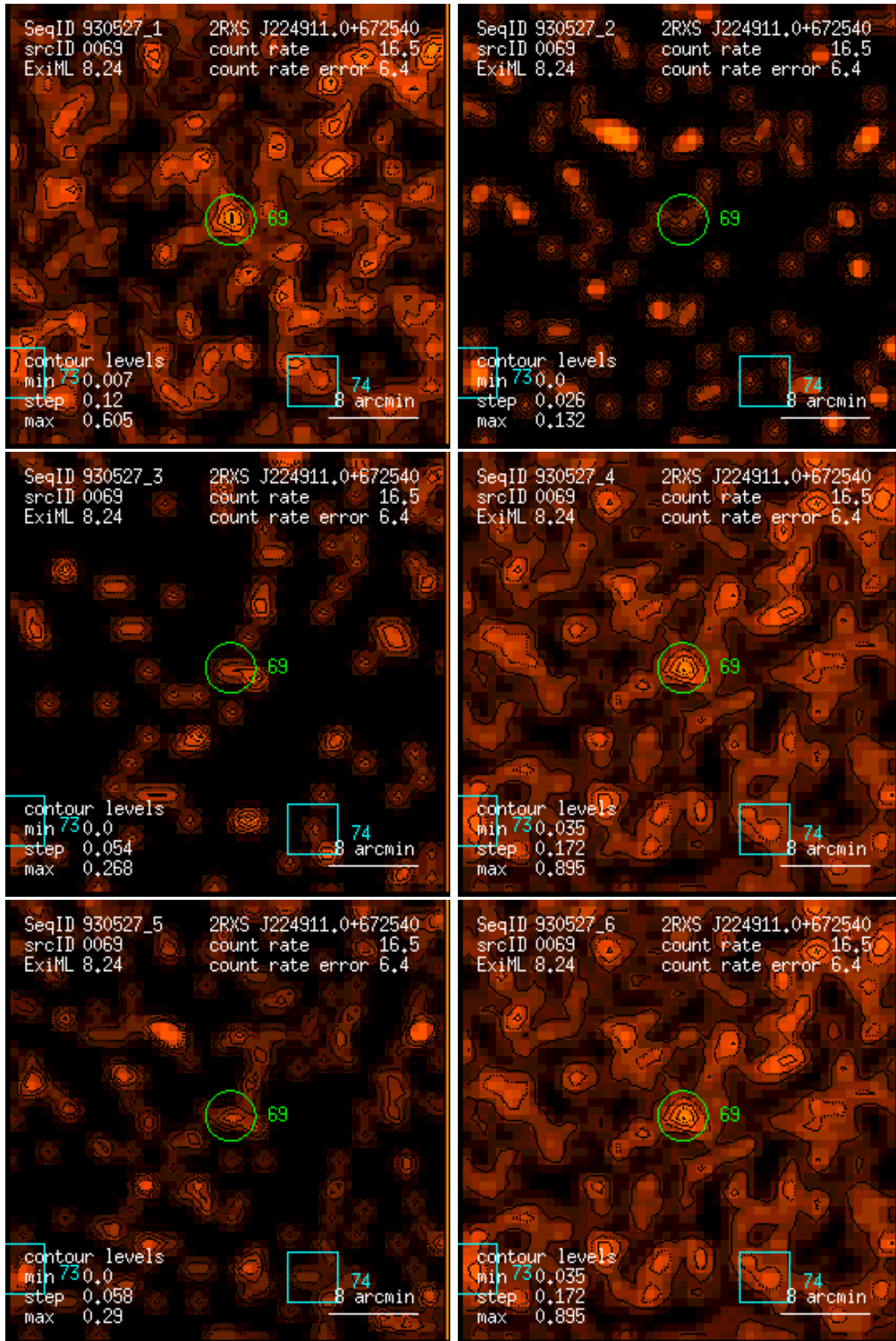
Figure 69: RASS 930527: detection 0069: band rate images, Gaussian filter: (1) PSPC channels 11 – 41, (2) 52 – 90, (3) 91 – 201, (4) 11 – 235, (5) 52 – 201, (6) 11 – 201. Broad band rates in counts/ks. Band rate contour levels in counts/ks/arcmin 2 .
