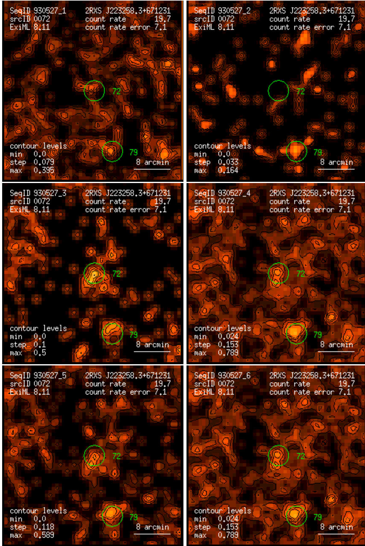
Figure 72: RASS 930527: detection 0072: band rate images, Gaussian filter: (1) PSPC channels 11 – 41, (2) 52 – 90, (3) 91 – 201, (4) 11 – 235, (5) 52 – 201, (6) 11 – 201. Broad band rates in counts/ks. Band rate contour levels in counts/ks/arcmin 2 .
