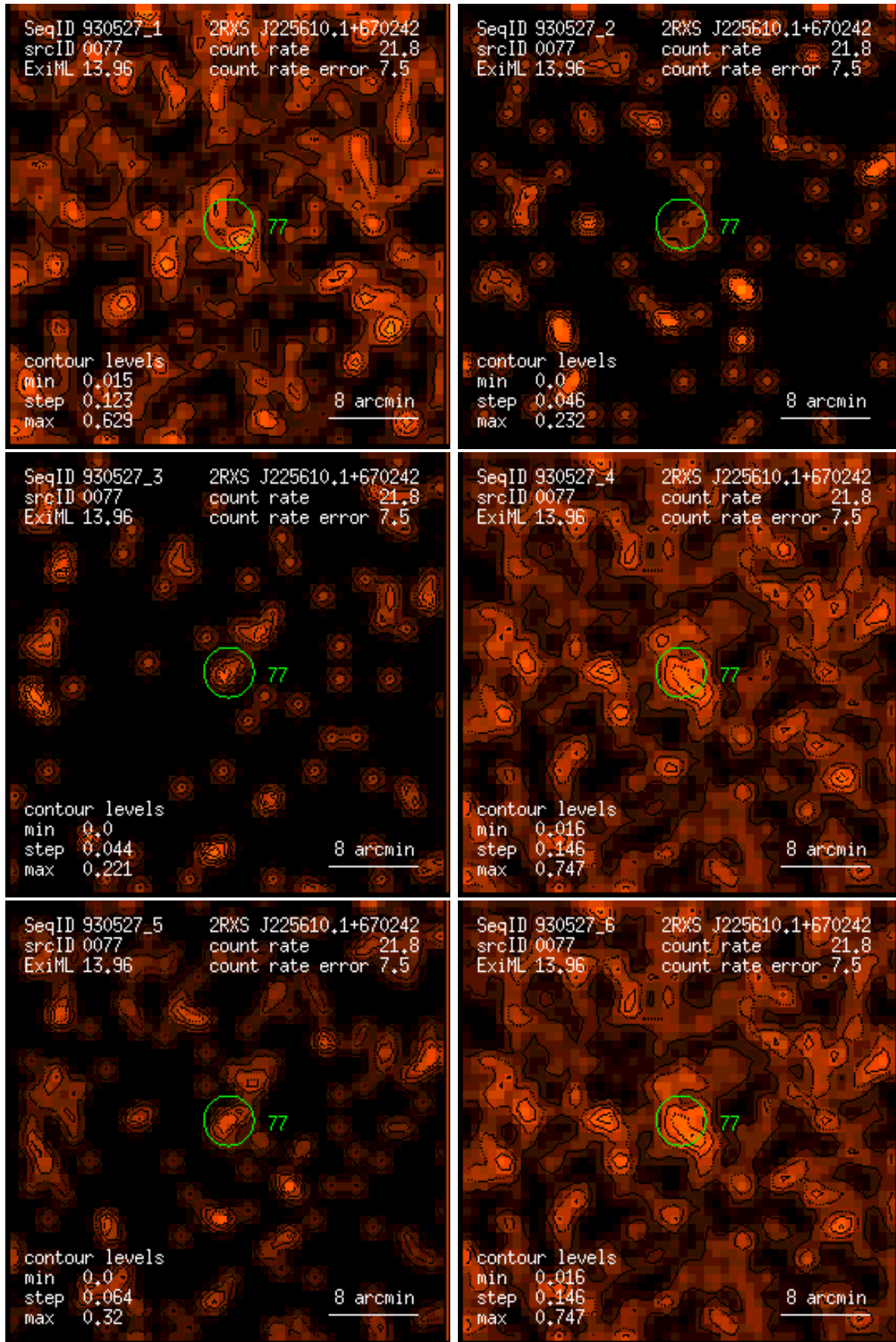
Figure 77: RASS 930527: detection 0077: band rate images, Gaussian filter: (1) PSPC channels 11 – 41, (2) 52 – 90, (3) 91 – 201, (4) 11 – 235, (5) 52 – 201, (6) 11 – 201. Broad band rates in counts/ks. Band rate contour levels in counts/ks/arcmin 2 .
