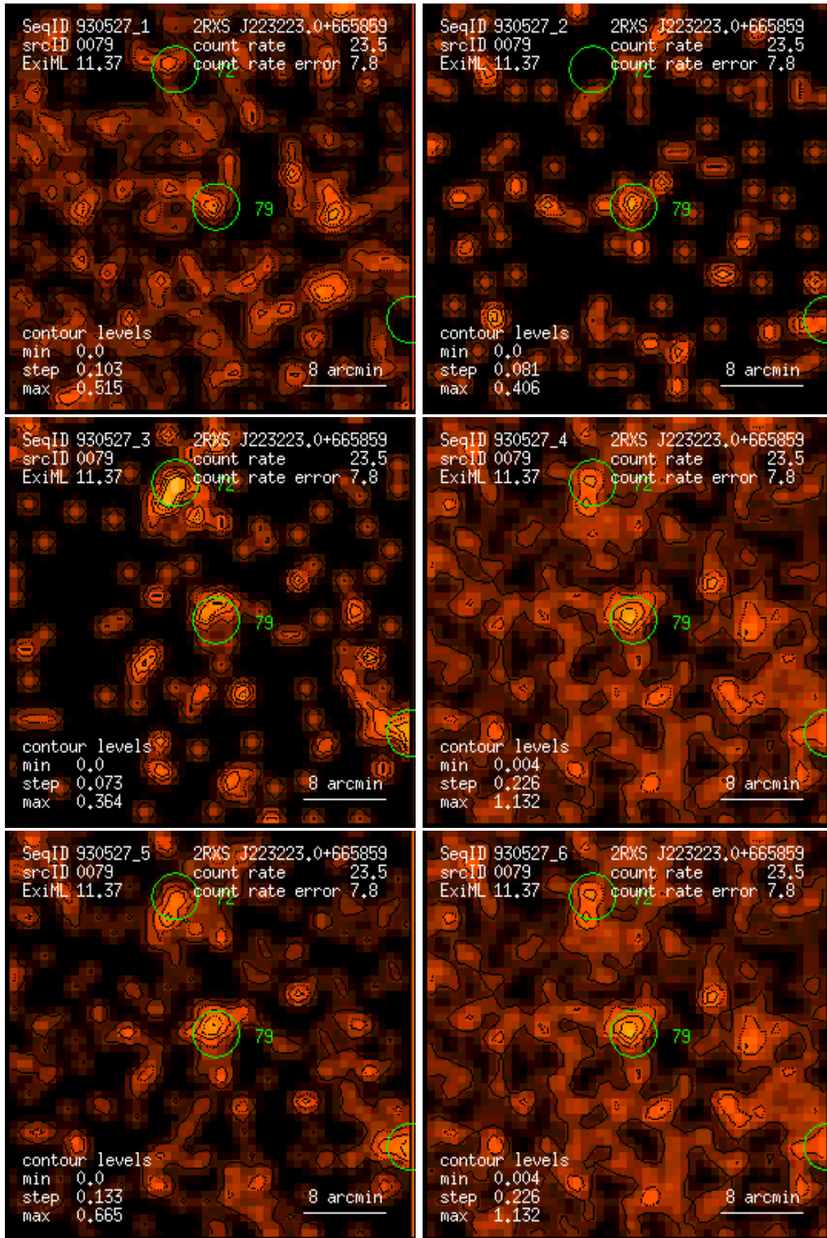
Figure 79: RASS 930527: detection 0079: band rate images, Gaussian filter: (1) PSPC channels 11 – 41, (2) 52 – 90, (3) 91 – 201, (4) 11 – 235, (5) 52 – 201, (6) 11 – 201. Broad band rates in counts/ks. Band rate contour levels in counts/ks/arcmin 2 .
