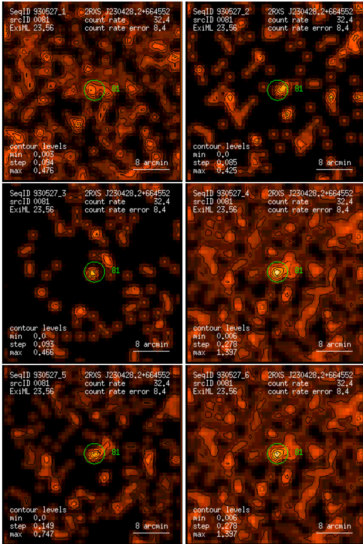
Figure 81: RASS 930527: detection 0081: band rate images, Gaussian filter: (1) PSPC channels 11 – 41, (2) 52 – 90, (3) 91 – 201, (4) 11 – 235, (5) 52 – 201, (6) 11 – 201. Broad band rates in counts/ks. Band rate contour levels in counts/ks/arcmin 2 .
