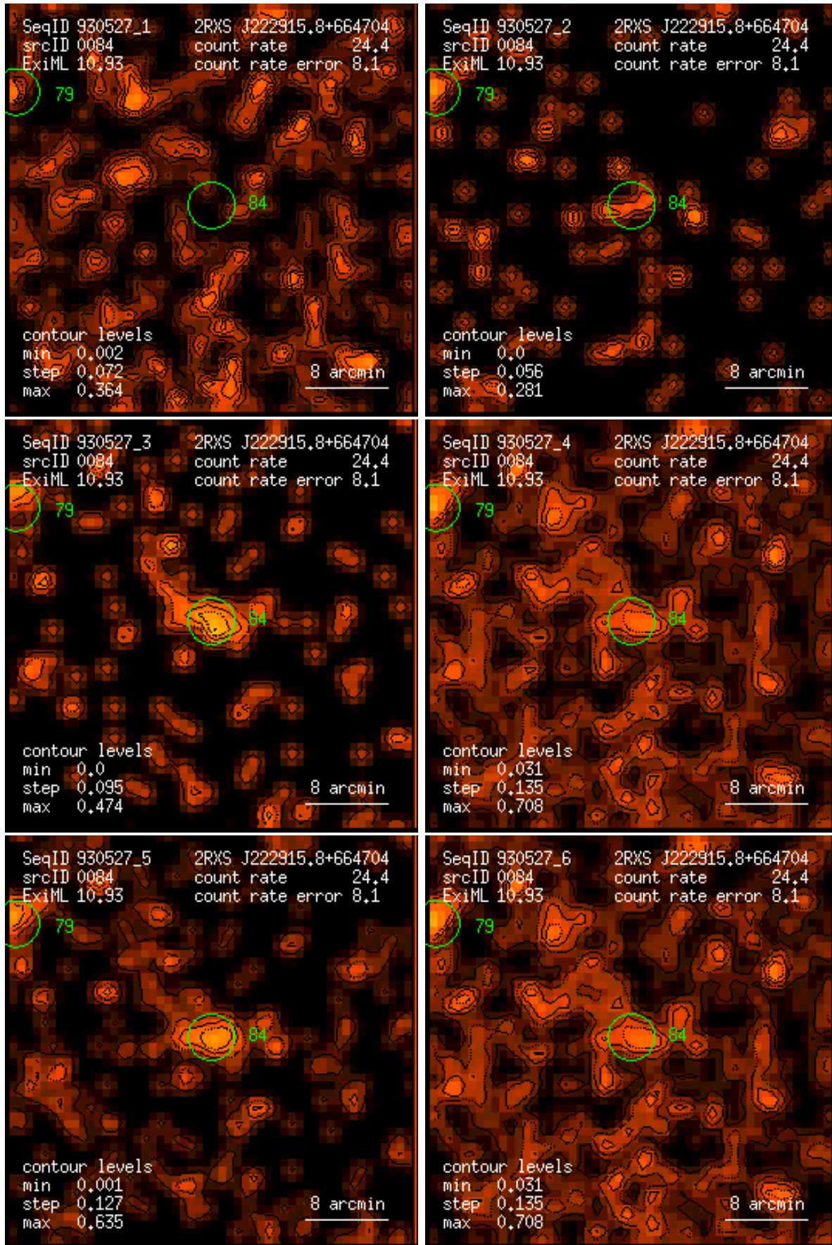
Figure 84: RASS 930527: detection 0084: band rate images, Gaussian filter: (1) PSPC channels 11 – 41, (2) 52 – 90, (3) 91 – 201, (4) 11 – 235, (5) 52 – 201, (6) 11 – 201. Broad band rates in counts/ks. Band rate contour levels in counts/ks/arcmin 2 .
