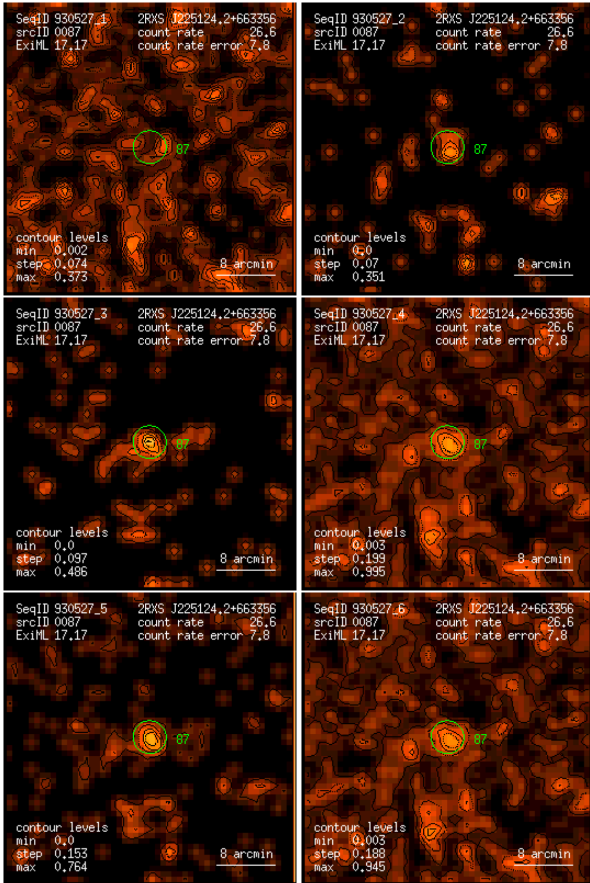
Figure 87: RASS 930527: detection 0087: band rate images, Gaussian filter: (1) PSPC channels 11 – 41, (2) 52 – 90, (3) 91 – 201, (4) 11 – 235, (5) 52 – 201, (6) 11 – 201. Broad band rates in counts/ks. Band rate contour levels in counts/ks/arcmin 2 .
