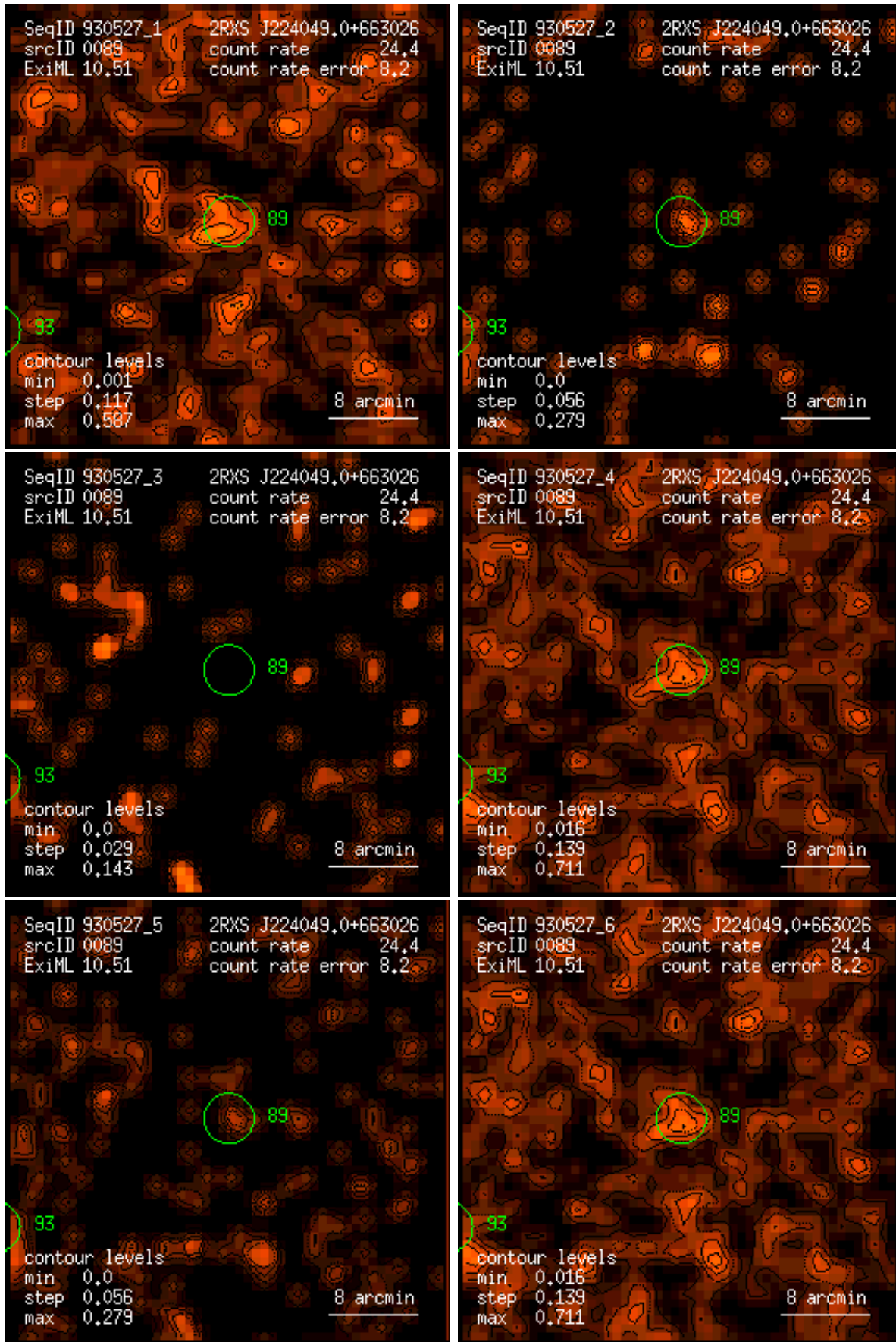
Figure 89: RASS 930527: detection 0089: band rate images, Gaussian filter: (1) PSPC channels 11 – 41, (2) 52 – 90, (3) 91 – 201, (4) 11 – 235, (5) 52 – 201, (6) 11 – 201. Broad band rates in counts/ks. Band rate contour levels in counts/ks/arcmin 2 .
