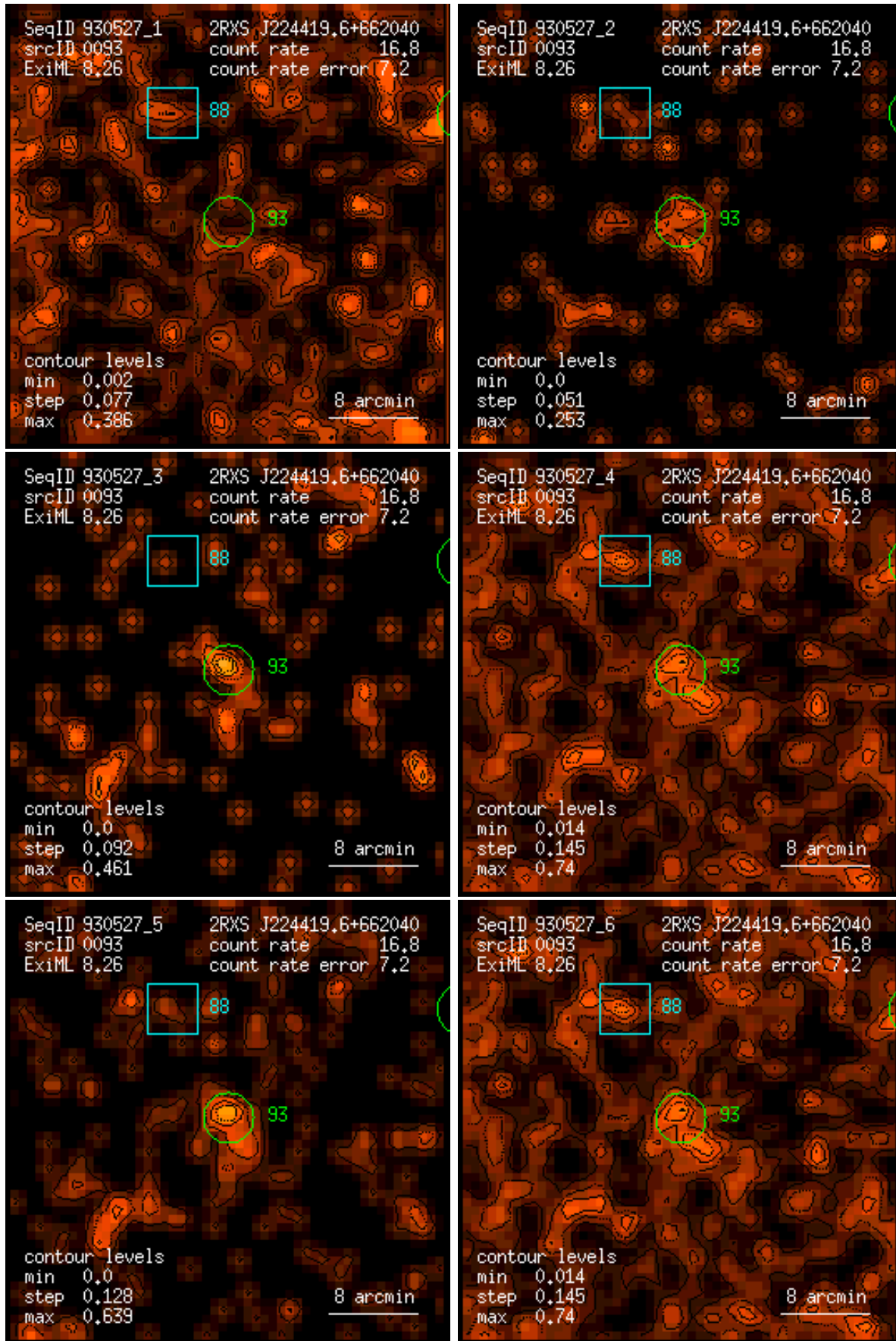
Figure 93: RASS 930527: detection 0093: band rate images, Gaussian filter: (1) PSPC channels 11 – 41, (2) 52 – 90, (3) 91 – 201, (4) 11 – 235, (5) 52 – 201, (6) 11 – 201. Broad band rates in counts/ks. Band rate contour levels in counts/ks/arcmin 2 .
