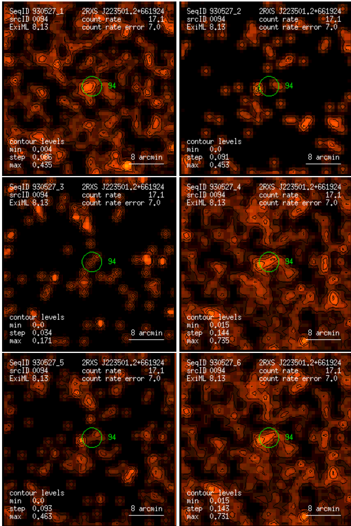
Figure 94: RASS 930527: detection 0094: band rate images, Gaussian filter: (1) PSPC channels 11 – 41, (2) 52 – 90, (3) 91 – 201, (4) 11 – 235, (5) 52 – 201, (6) 11 – 201. Broad band rates in counts/ks. Band rate contour levels in counts/ks/arcmin 2 .
