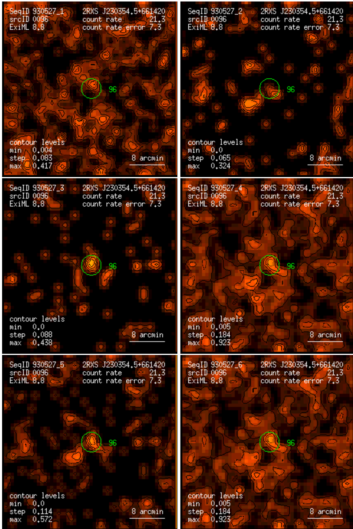
Figure 96: RASS 930527: detection 0096: band rate images, Gaussian filter: (1) PSPC channels 11 – 41, (2) 52 – 90, (3) 91 – 201, (4) 11 – 235, (5) 52 – 201, (6) 11 – 201. Broad band rates in counts/ks. Band rate contour levels in counts/ks/arcmin 2 .
