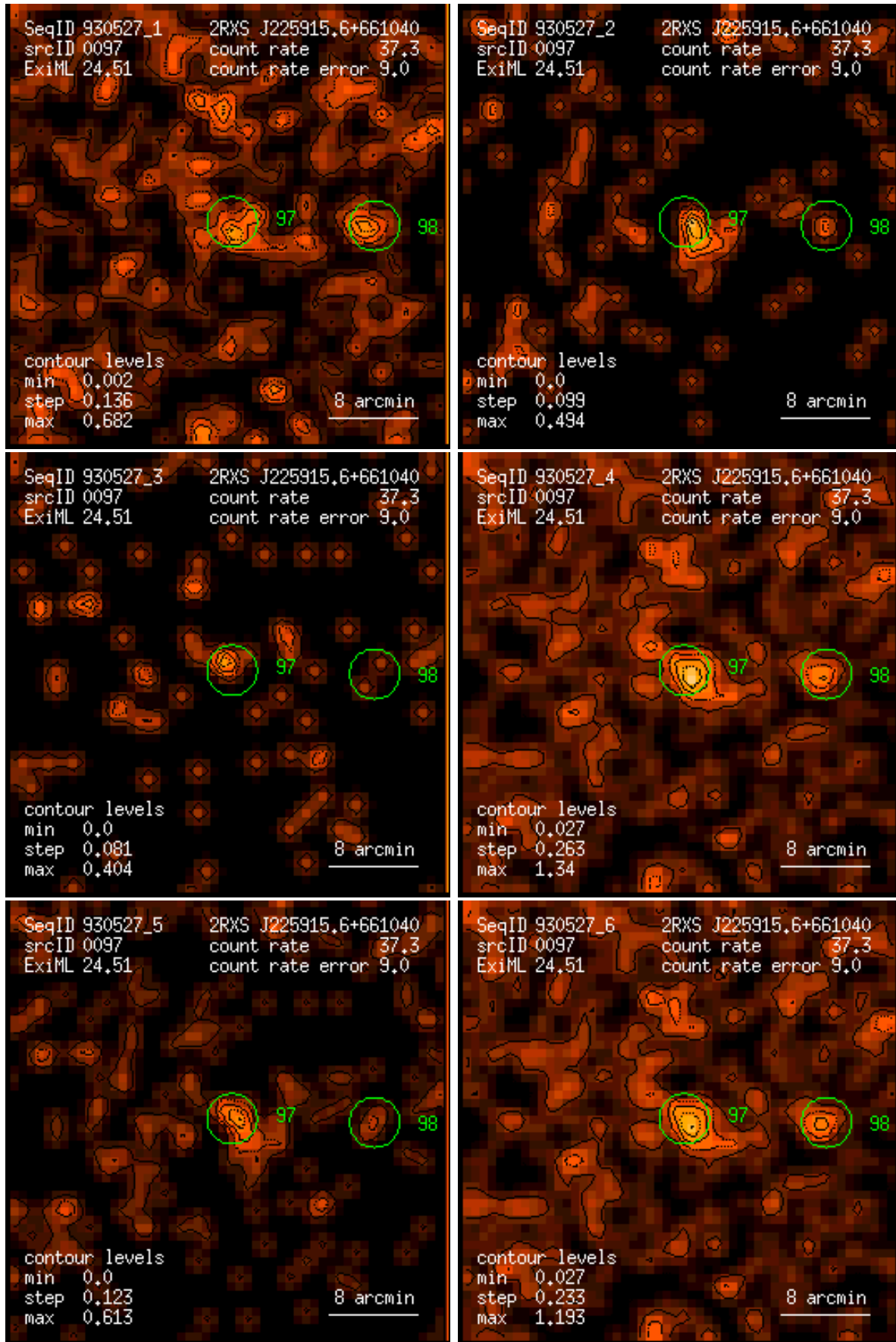
Figure 97: RASS 930527: detection 0097: band rate images, Gaussian filter: (1) PSPC channels 11 – 41, (2) 52 – 90, (3) 91 – 201, (4) 11 – 235, (5) 52 – 201, (6) 11 – 201. Broad band rates in counts/ks. Band rate contour levels in counts/ks/arcmin 2 .
