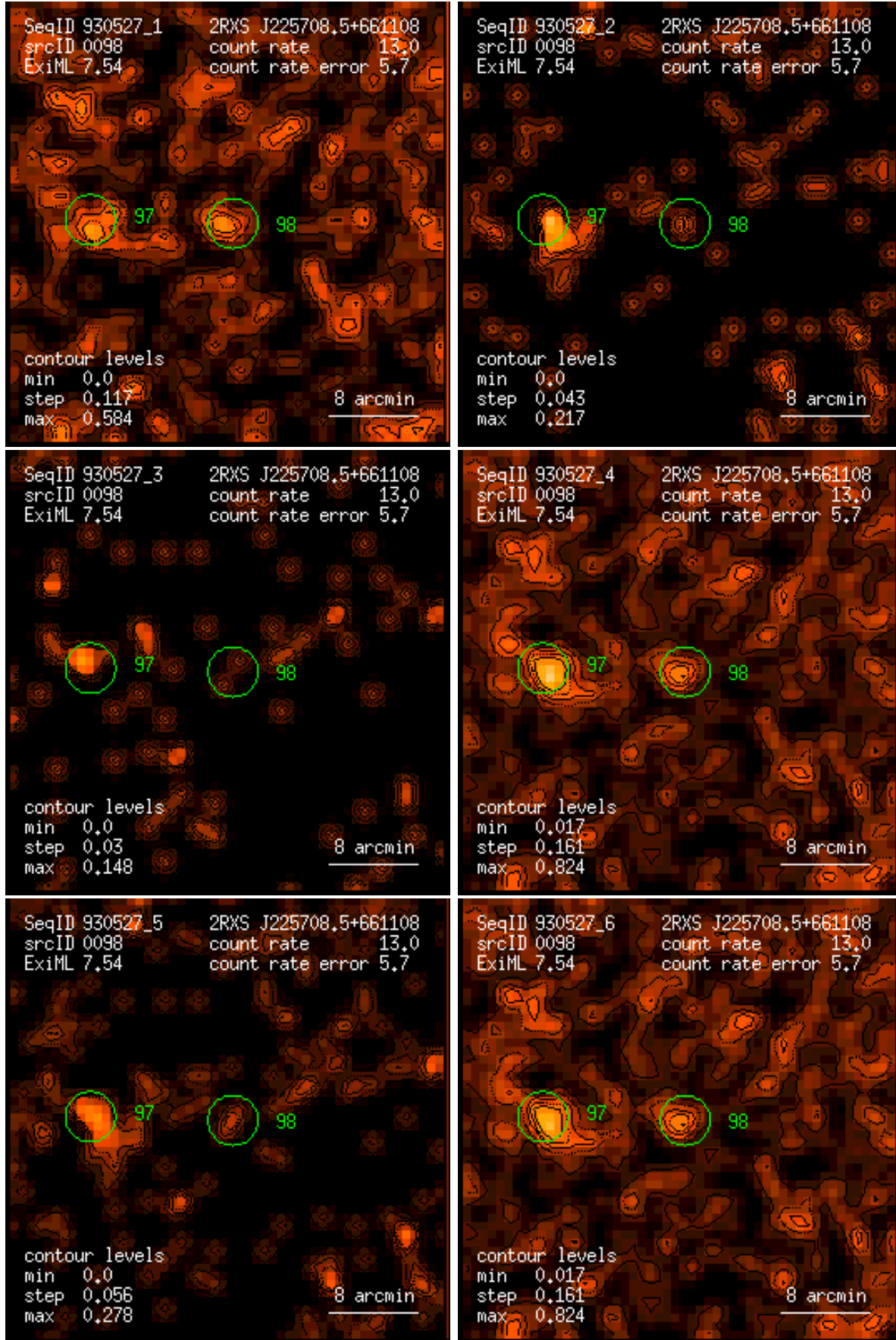
Figure 98: RASS 930527: detection 0098: band rate images, Gaussian filter: (1) PSPC channels 11 – 41, (2) 52 – 90, (3) 91 – 201, (4) 11 – 235, (5) 52 – 201, (6) 11 – 201. Broad band rates in counts/ks. Band rate contour levels in counts/ks/arcmin 2 .
