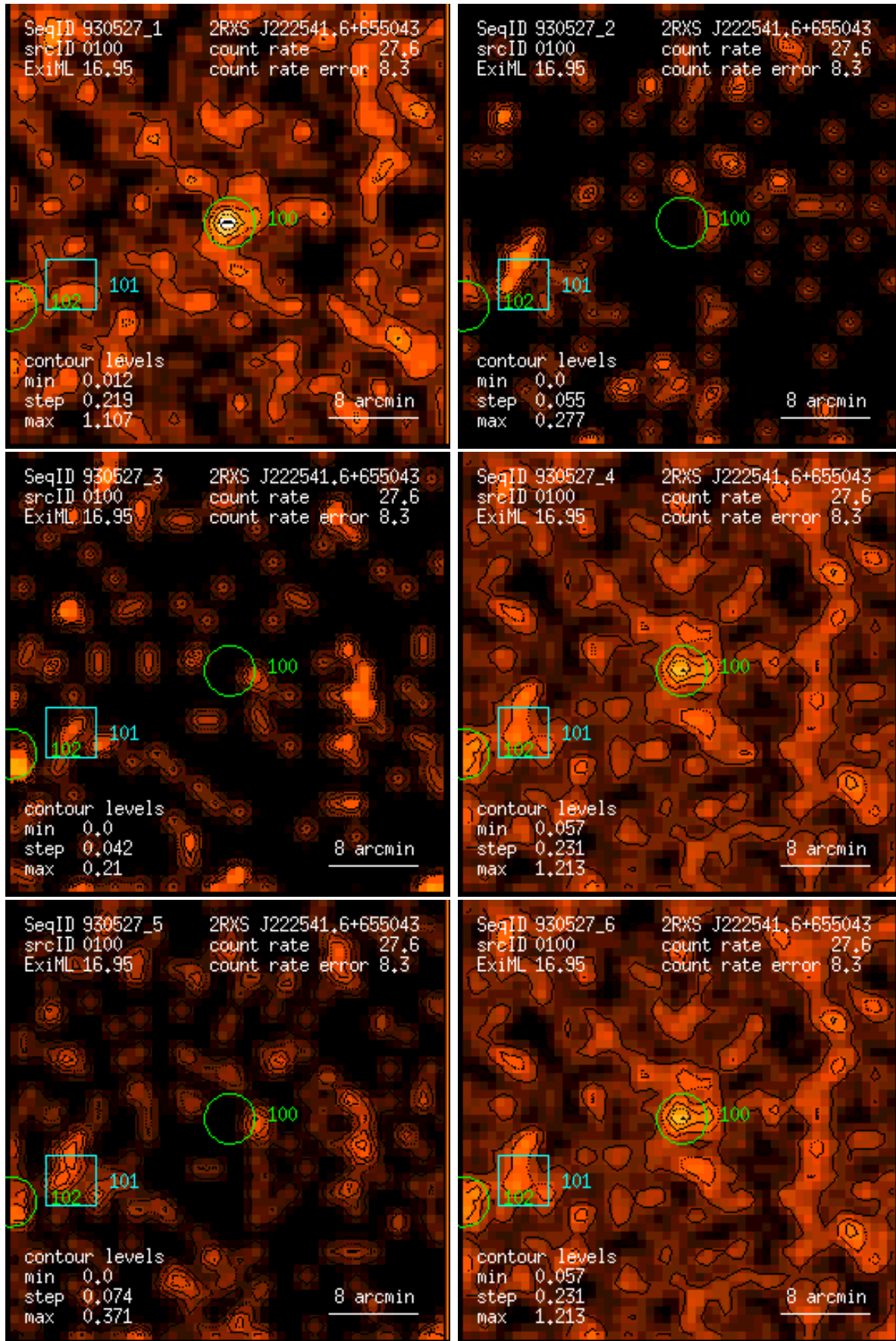
Figure 100: RASS 930527: detection 0100: band rate images, Gaussian filter: (1) PSPC channels 11 – 41, (2) 52 – 90, (3) 91 – 201, (4) 11 – 235, (5) 52 – 201, (6) 11 – 201. Broad band rates in counts/ks. Band rate contour levels in counts/ks/arcmin 2 .
