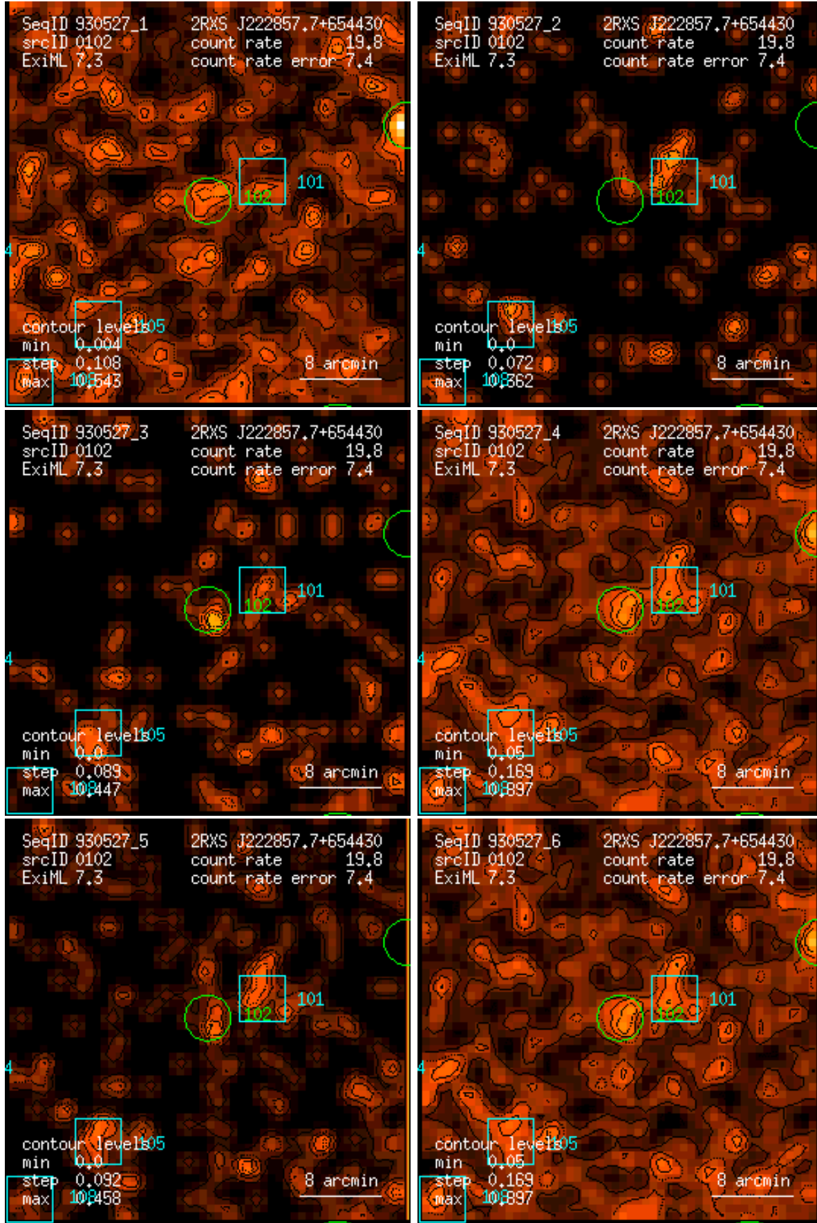
Figure 102: RASS 930527: detection 0102: band rate images, Gaussian filter: (1) PSPC channels 11 – 41, (2) 52 – 90, (3) 91 – 201, (4) 11 – 235, (5) 52 – 201, (6) 11 – 201. Broad band rates in counts/ks. Band rate contour levels in counts/ks/arcmin 2 .
