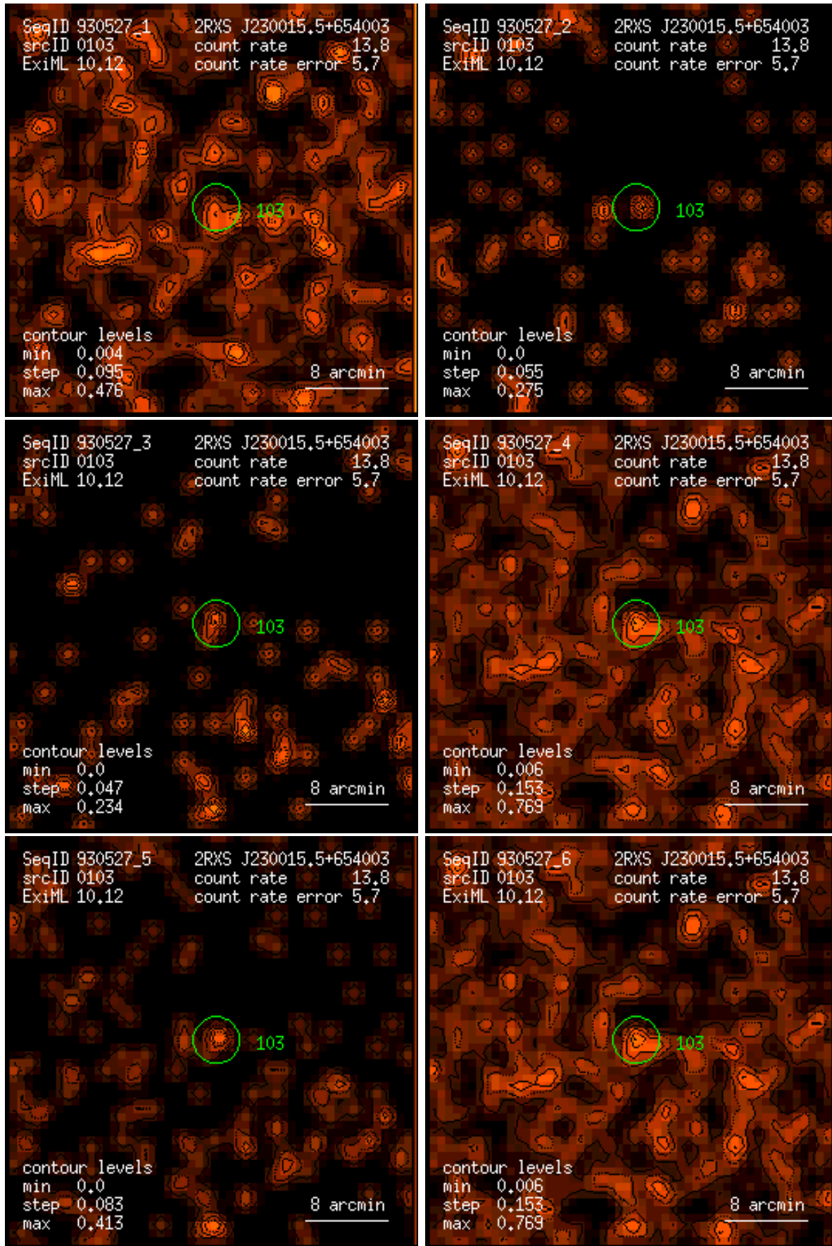
Figure 103: RASS 930527: detection 0103: band rate images, Gaussian filter: (1) PSPC channels 11 – 41, (2) 52 – 90, (3) 91 – 201, (4) 11 – 235, (5) 52 – 201, (6) 11 – 201. Broad band rates in counts/ks. Band rate contour levels in counts/ks/arcmin 2 .
