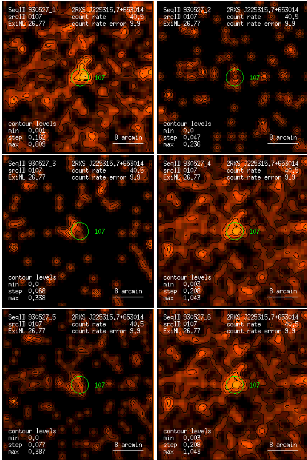
Figure 107: RASS 930527: detection 0107: band rate images, Gaussian filter: (1) PSPC channels 11 – 41, (2) 52 – 90, (3) 91 – 201, (4) 11 – 235, (5) 52 – 201, (6) 11 – 201. Broad band rates in counts/ks. Band rate contour levels in counts/ks/arcmin 2 .
