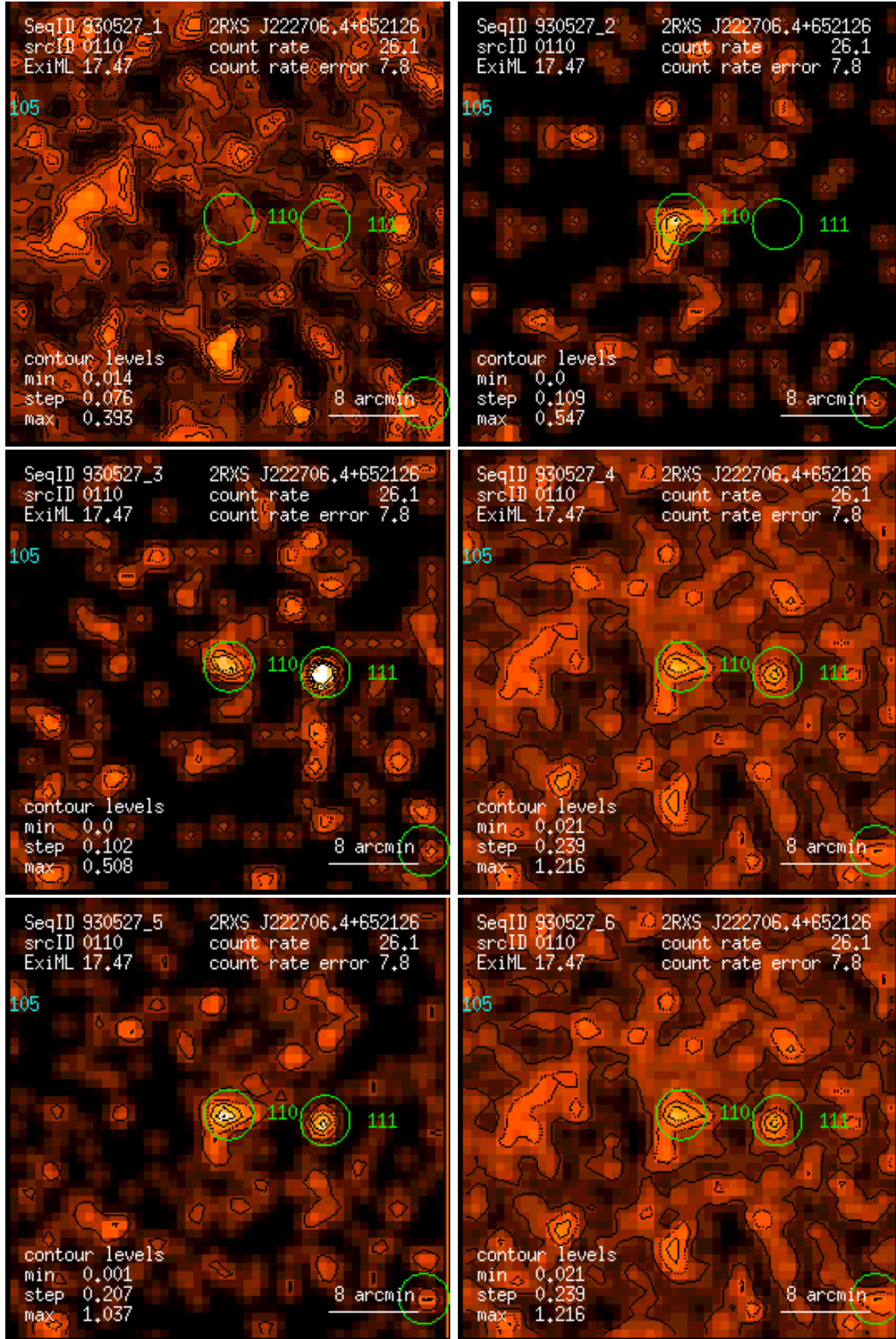
Figure 110: RASS 930527: detection 0110: band rate images, Gaussian filter: (1) PSPC channels 11 – 41, (2) 52 – 90, (3) 91 – 201, (4) 11 – 235, (5) 52 – 201, (6) 11 – 201. Broad band rates in counts/ks. Band rate contour levels in counts/ks/arcmin 2 .
