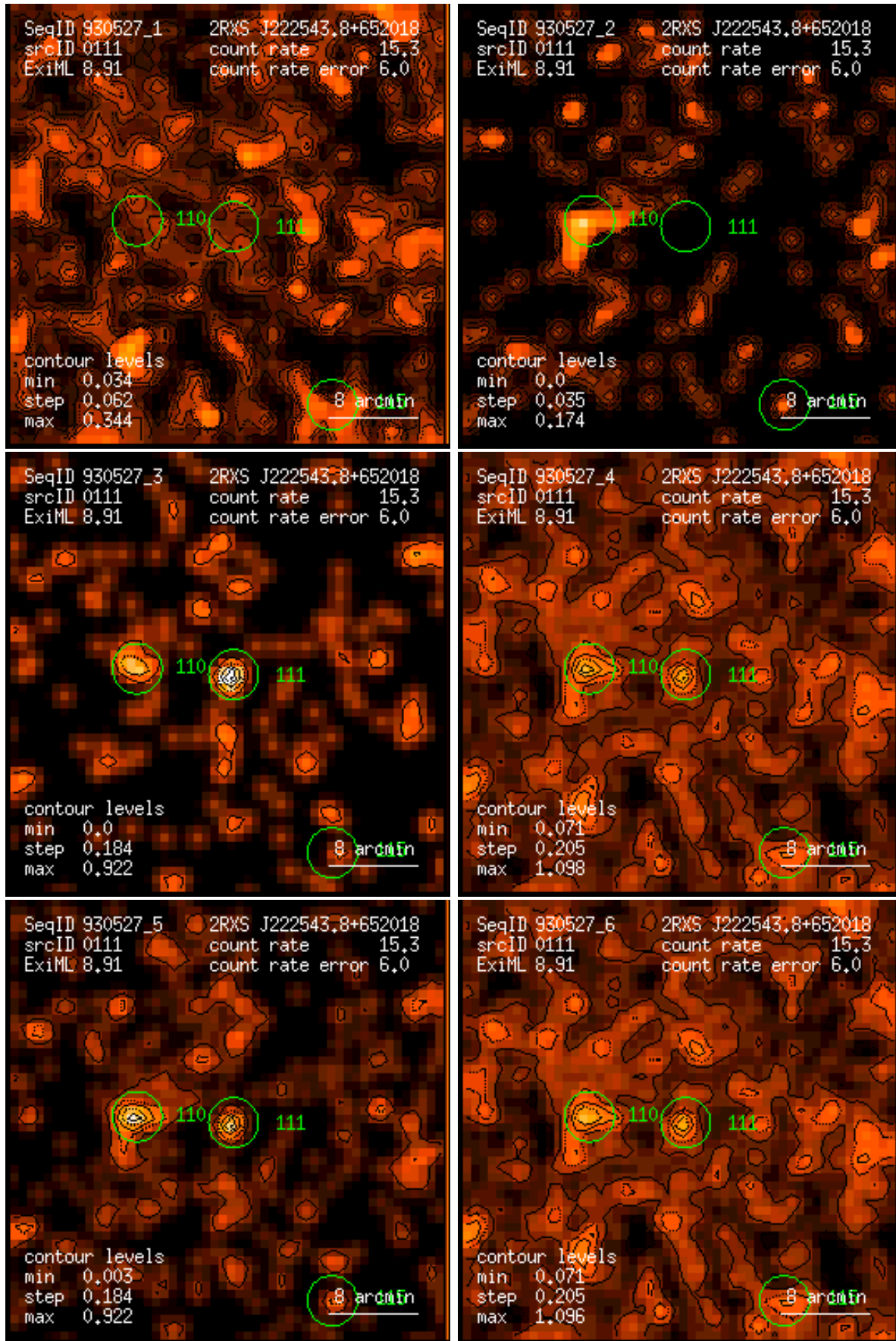
Figure 111: RASS 930527: detection 0111: band rate images, Gaussian filter: (1) PSPC channels 11 – 41, (2) 52 – 90, (3) 91 – 201, (4) 11 – 235, (5) 52 – 201, (6) 11 – 201. Broad band rates in counts/ks. Band rate contour levels in counts/ks/arcmin 2 .
