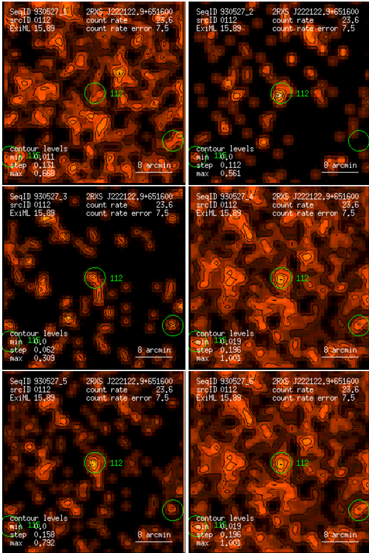
Figure 112: RASS 930527: detection 0112: band rate images, Gaussian filter: (1) PSPC channels 11 – 41, (2) 52 – 90, (3) 91 – 201, (4) 11 – 235, (5) 52 – 201, (6) 11 – 201. Broad band rates in counts/ks. Band rate contour levels in counts/ks/arcmin 2 .
