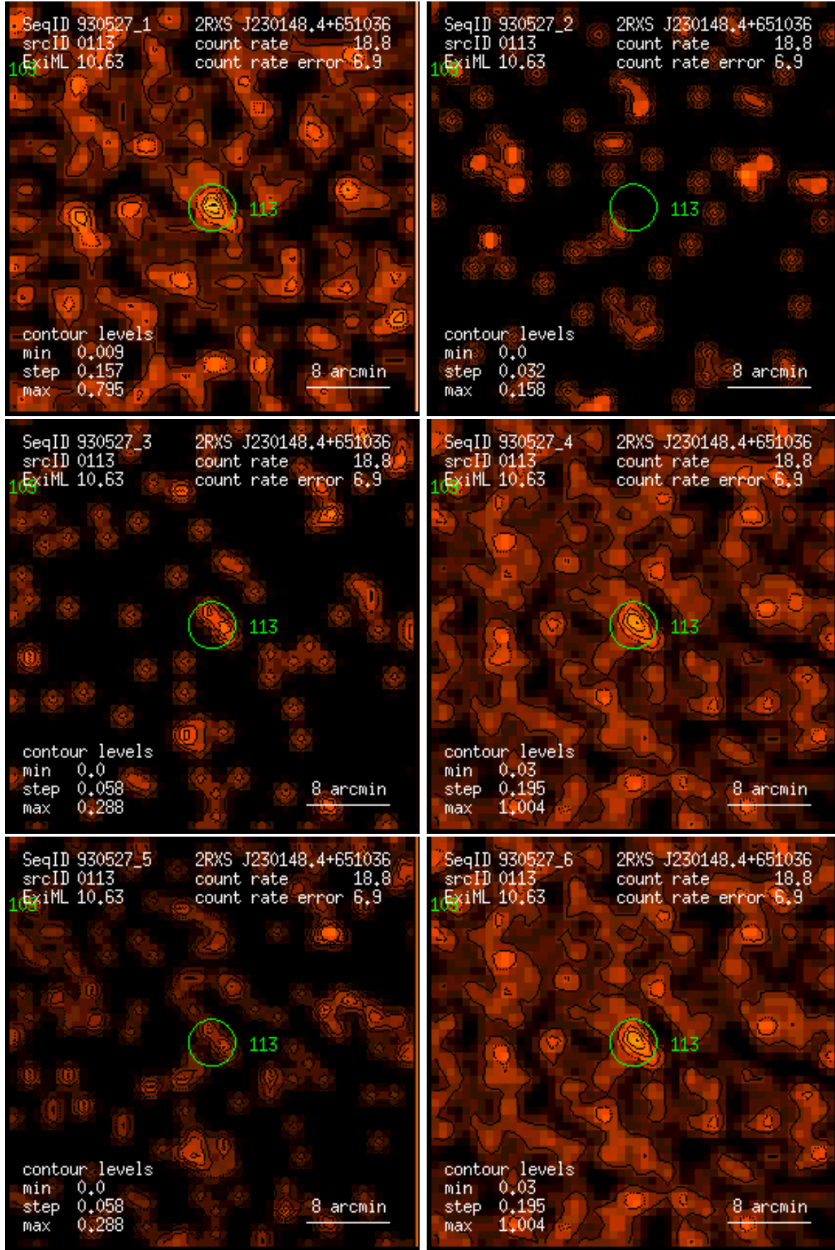
Figure 113: RASS 930527: detection 0113: band rate images, Gaussian filter: (1) PSPC channels 11 – 41, (2) 52 – 90, (3) 91 – 201, (4) 11 – 235, (5) 52 – 201, (6) 11 – 201. Broad band rates in counts/ks. Band rate contour levels in counts/ks/arcmin 2 .
