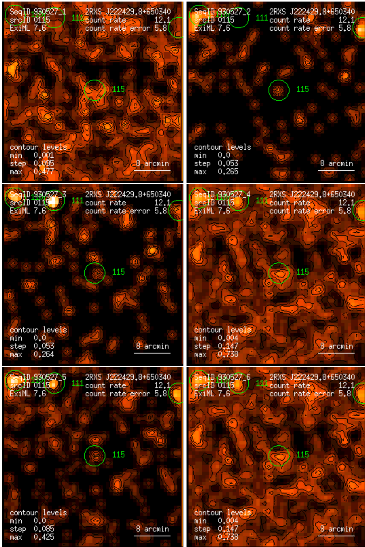
Figure 115: RASS 930527: detection 0115: band rate images, Gaussian filter: (1) PSPC channels 11 – 41, (2) 52 – 90, (3) 91 – 201, (4) 11 – 235, (5) 52 – 201, (6) 11 – 201. Broad band rates in counts/ks. Band rate contour levels in counts/ks/arcmin 2 .
