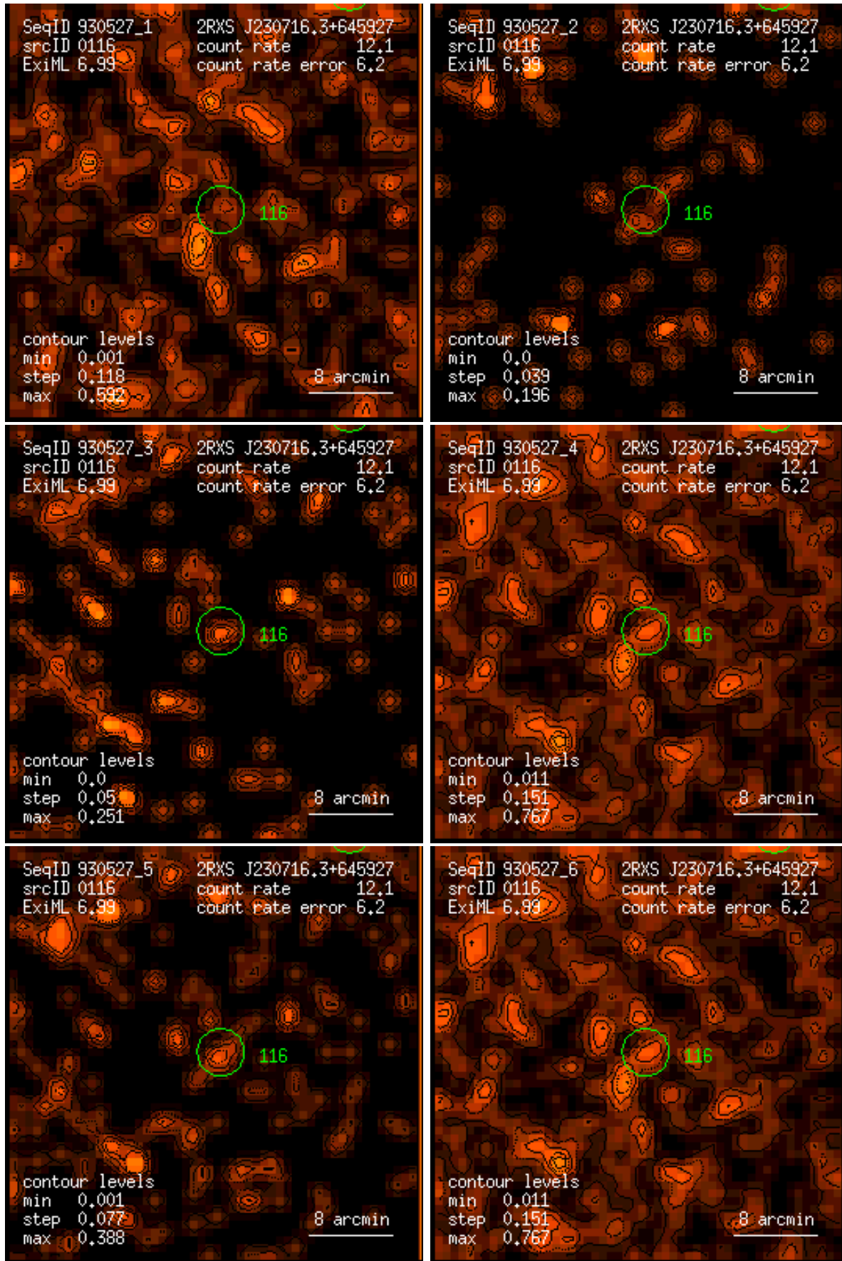
Figure 116: RASS 930527: detection 0116: band rate images, Gaussian filter: (1) PSPC channels 11 – 41, (2) 52 – 90, (3) 91 – 201, (4) 11 – 235, (5) 52 – 201, (6) 11 – 201. Broad band rates in counts/ks. Band rate contour levels in counts/ks/arcmin 2 .
