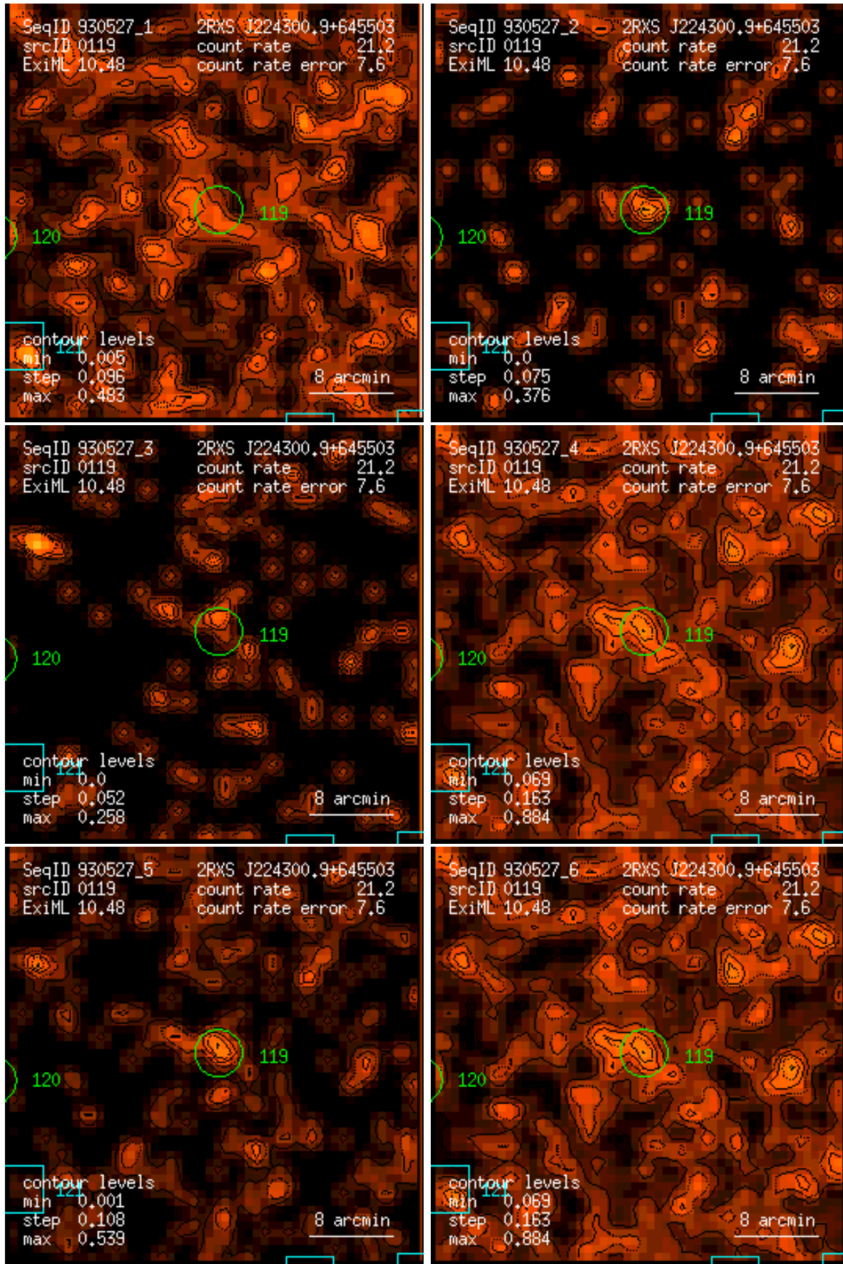
Figure 119: RASS 930527: detection 0119: band rate images, Gaussian filter: (1) PSPC channels 11 – 41, (2) 52 – 90, (3) 91 – 201, (4) 11 – 235, (5) 52 – 201, (6) 11 – 201. Broad band rates in counts/ks. Band rate contour levels in counts/ks/arcmin 2 .
