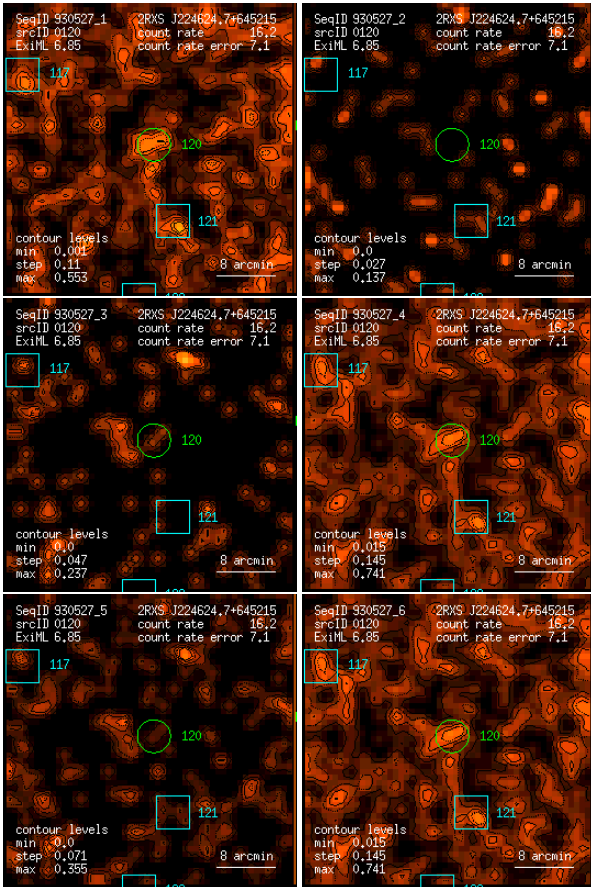
Figure 120: RASS 930527: detection 0120: band rate images, Gaussian filter: (1) PSPC channels 11 – 41, (2) 52 – 90, (3) 91 – 201, (4) 11 – 235, (5) 52 – 201, (6) 11 – 201. Broad band rates in counts/ks. Band rate contour levels in counts/ks/arcmin 2 .
