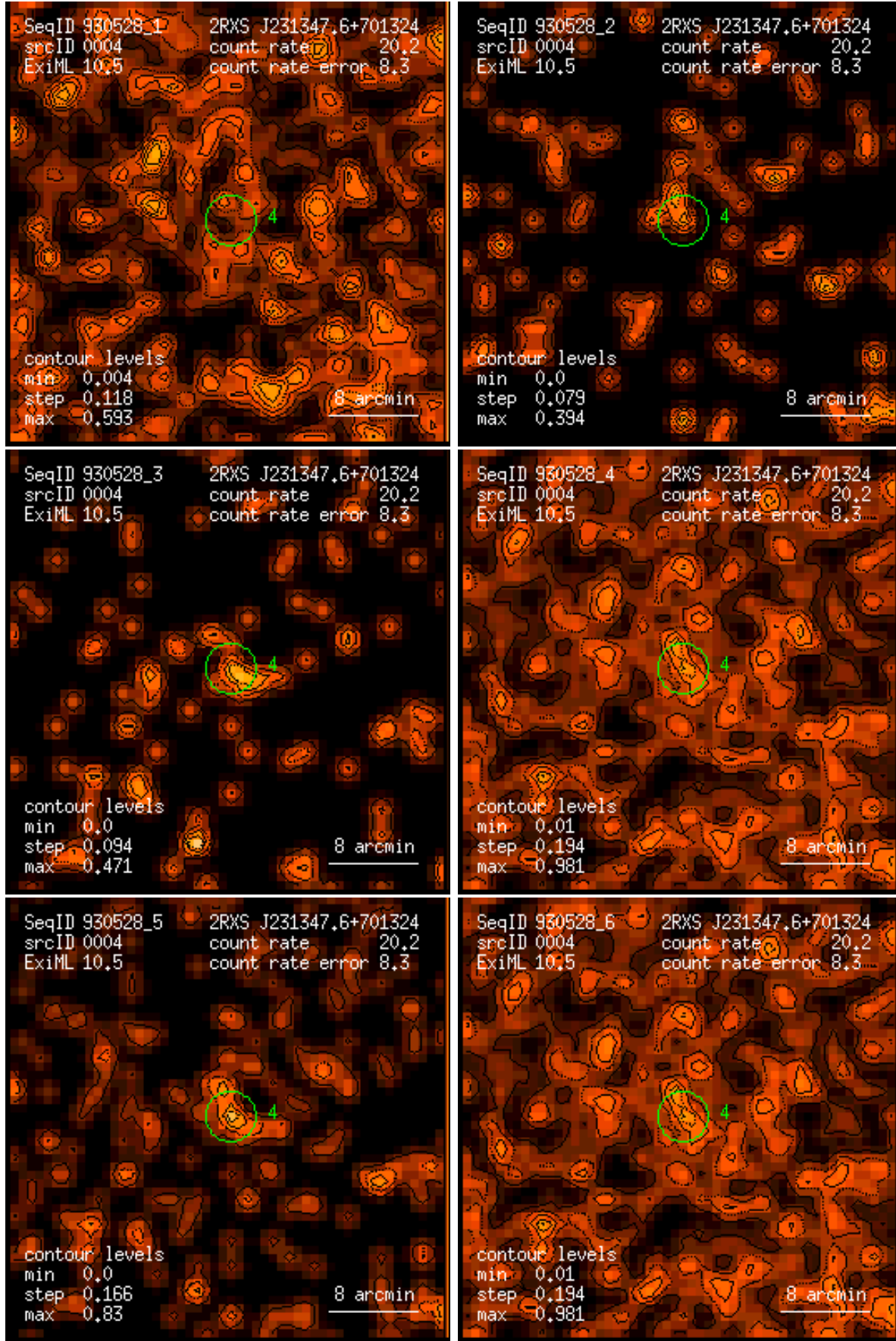
Figure 4: RASS 930528: detection 0004: band rate images, Gaussian filter: (1) PSPC channels 11 – 41, (2) 52 – 90, (3) 91 – 201, (4) 11 – 235, (5) 52 – 201, (6) 11 – 201. Broad band rates in counts/ks. Band rate contour levels in counts/ks/arcmin 2 .
