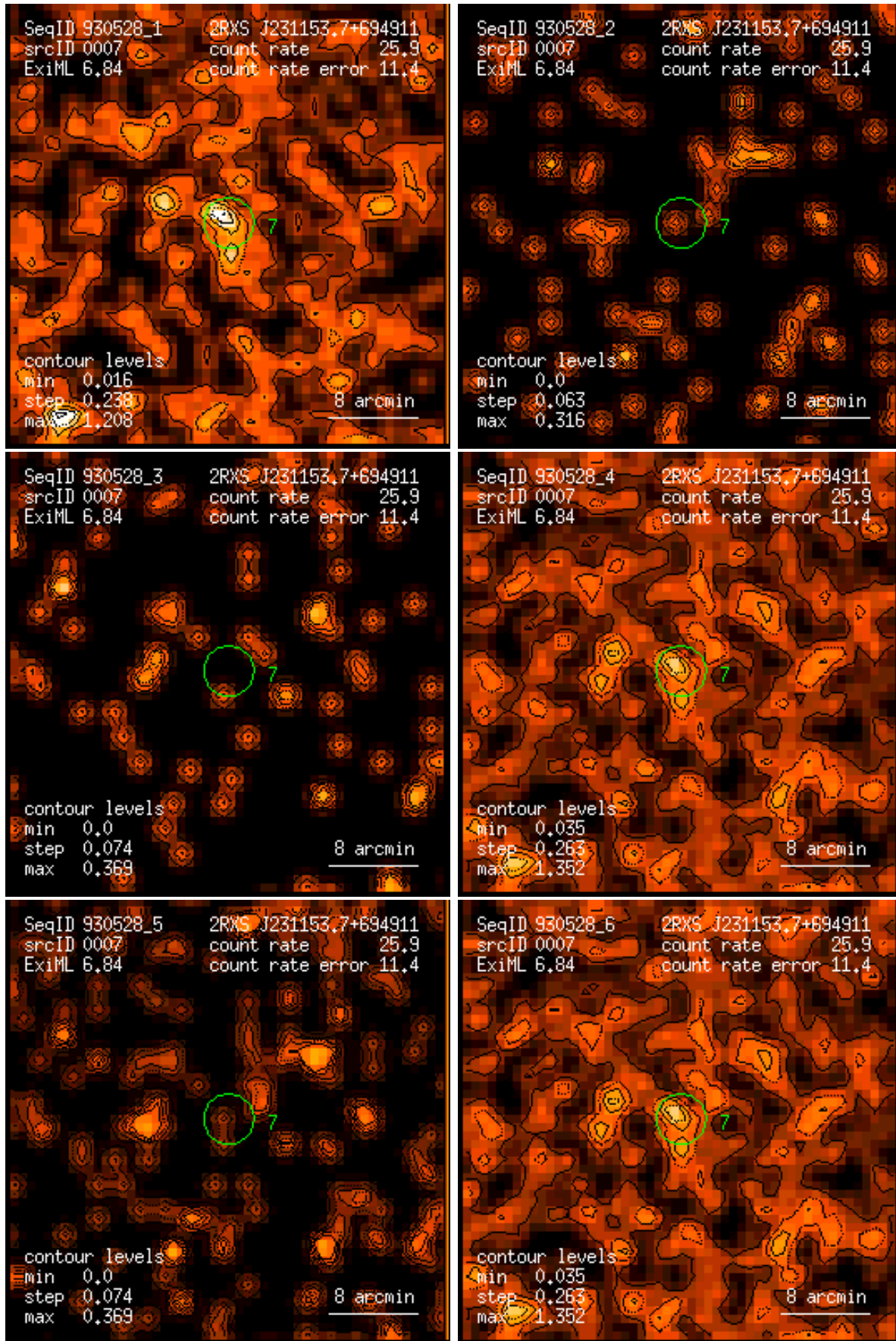
Figure 7: RASS 930528: detection 0007: band rate images, Gaussian filter: (1) PSPC channels 11 – 41, (2) 52 – 90, (3) 91 – 201, (4) 11 – 235, (5) 52 – 201, (6) 11 – 201. Broad band rates in counts/ks. Band rate contour levels in counts/ks/arcmin 2 .
