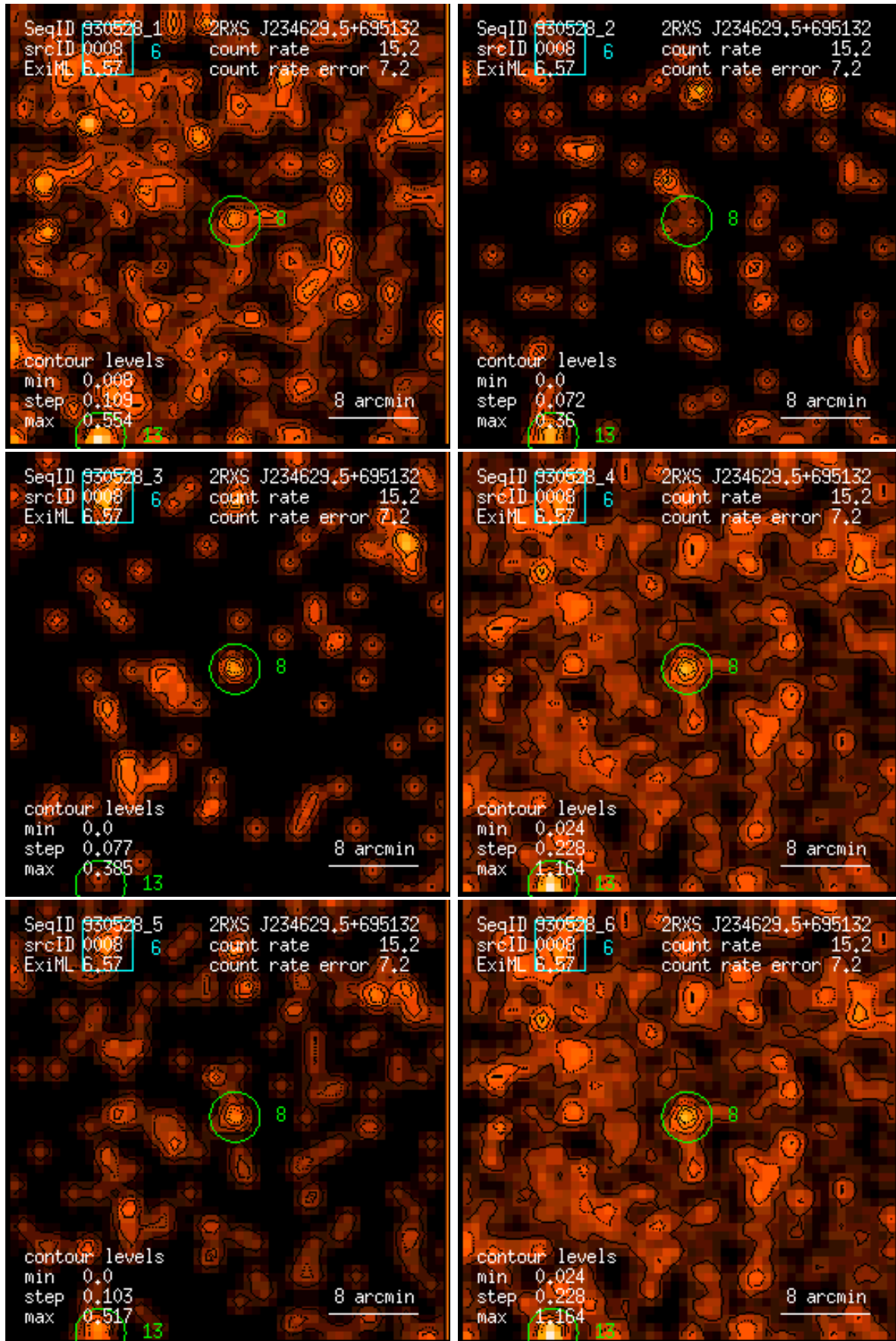
Figure 8: RASS 930528: detection 0008: band rate images, Gaussian filter: (1) PSPC channels 11 – 41, (2) 52 – 90, (3) 91 – 201, (4) 11 – 235, (5) 52 – 201, (6) 11 – 201. Broad band rates in counts/ks. Band rate contour levels in counts/ks/arcmin 2 .
