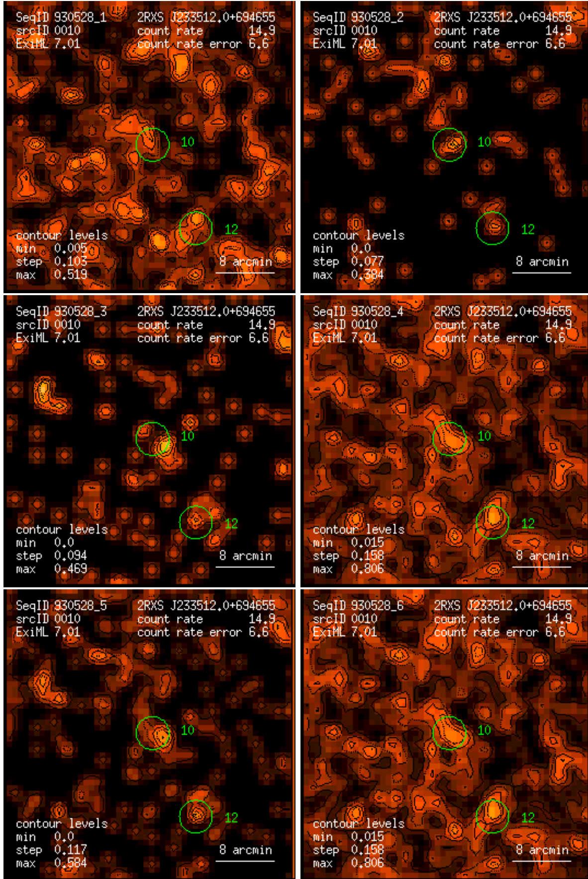
Figure 10: RASS 930528: detection 0010: band rate images, Gaussian filter: (1) PSPC channels 11 – 41, (2) 52 – 90, (3) 91 – 201, (4) 11 – 235, (5) 52 – 201, (6) 11 – 201. Broad band rates in counts/ks. Band rate contour levels in counts/ks/arcmin 2 .
