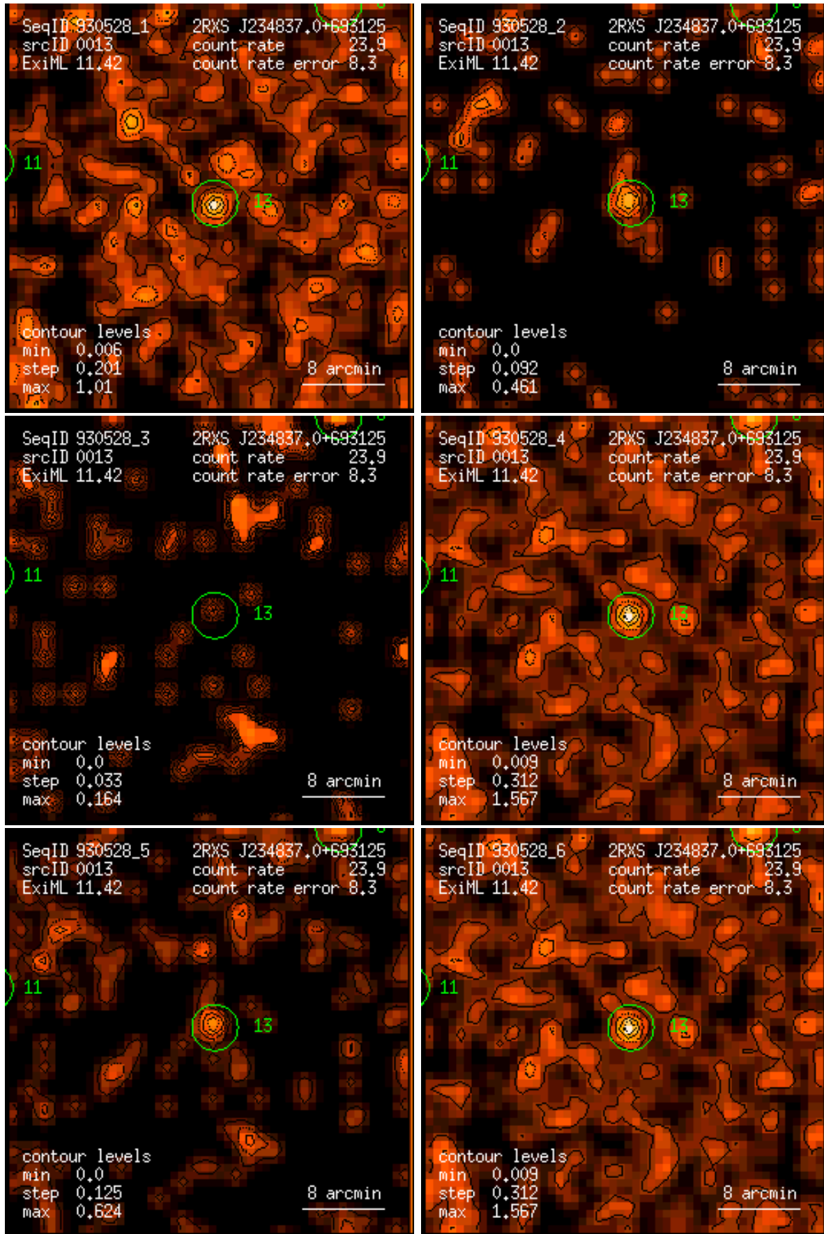
Figure 13: RASS 930528: detection 0013: band rate images, Gaussian filter: (1) PSPC channels 11 – 41, (2) 52 – 90, (3) 91 – 201, (4) 11 – 235, (5) 52 – 201, (6) 11 – 201. Broad band rates in counts/ks. Band rate contour levels in counts/ks/arcmin 2 .
