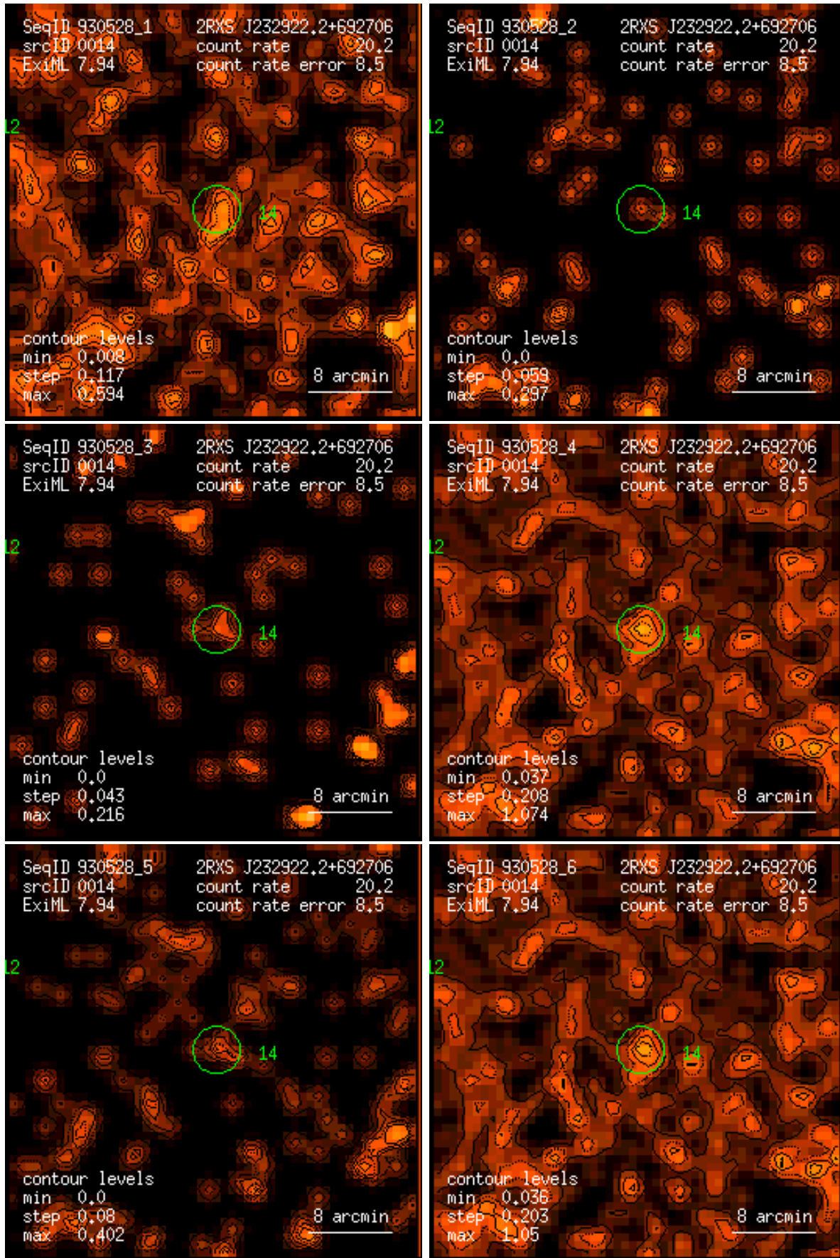
Figure 14: RASS 930528: detection 0014: band rate images, Gaussian filter: (1) PSPC channels 11 – 41, (2) 52 – 90, (3) 91 – 201, (4) 11 – 235, (5) 52 – 201, (6) 11 – 201. Broad band rates in counts/ks. Band rate contour levels in counts/ks/arcmin 2 .
