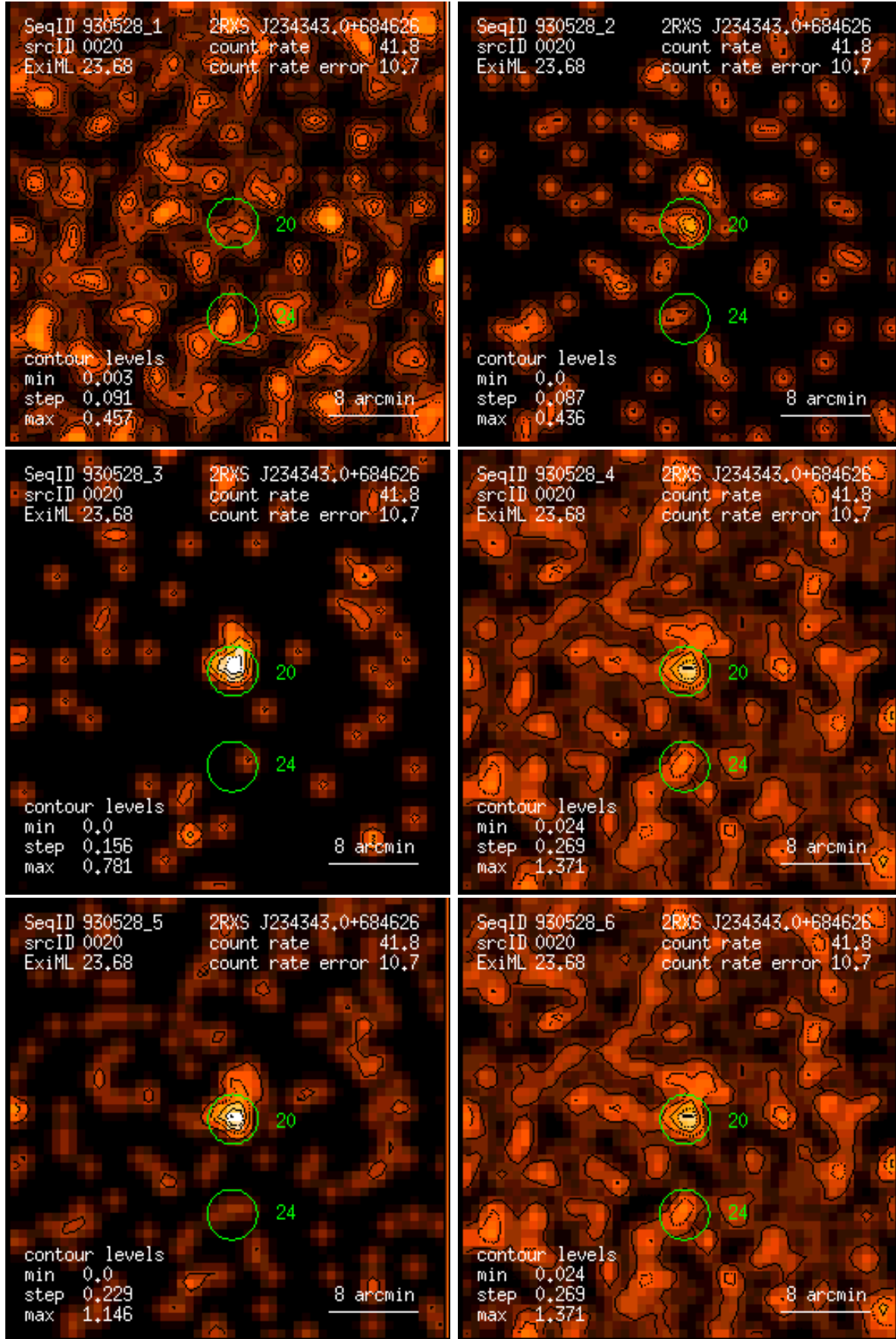
Figure 20: RASS 930528: detection 0020: band rate images, Gaussian filter: (1) PSPC channels 11 – 41, (2) 52 – 90, (3) 91 – 201, (4) 11 – 235, (5) 52 – 201, (6) 11 – 201. Broad band rates in counts/ks. Band rate contour levels in counts/ks/arcmin 2 .
