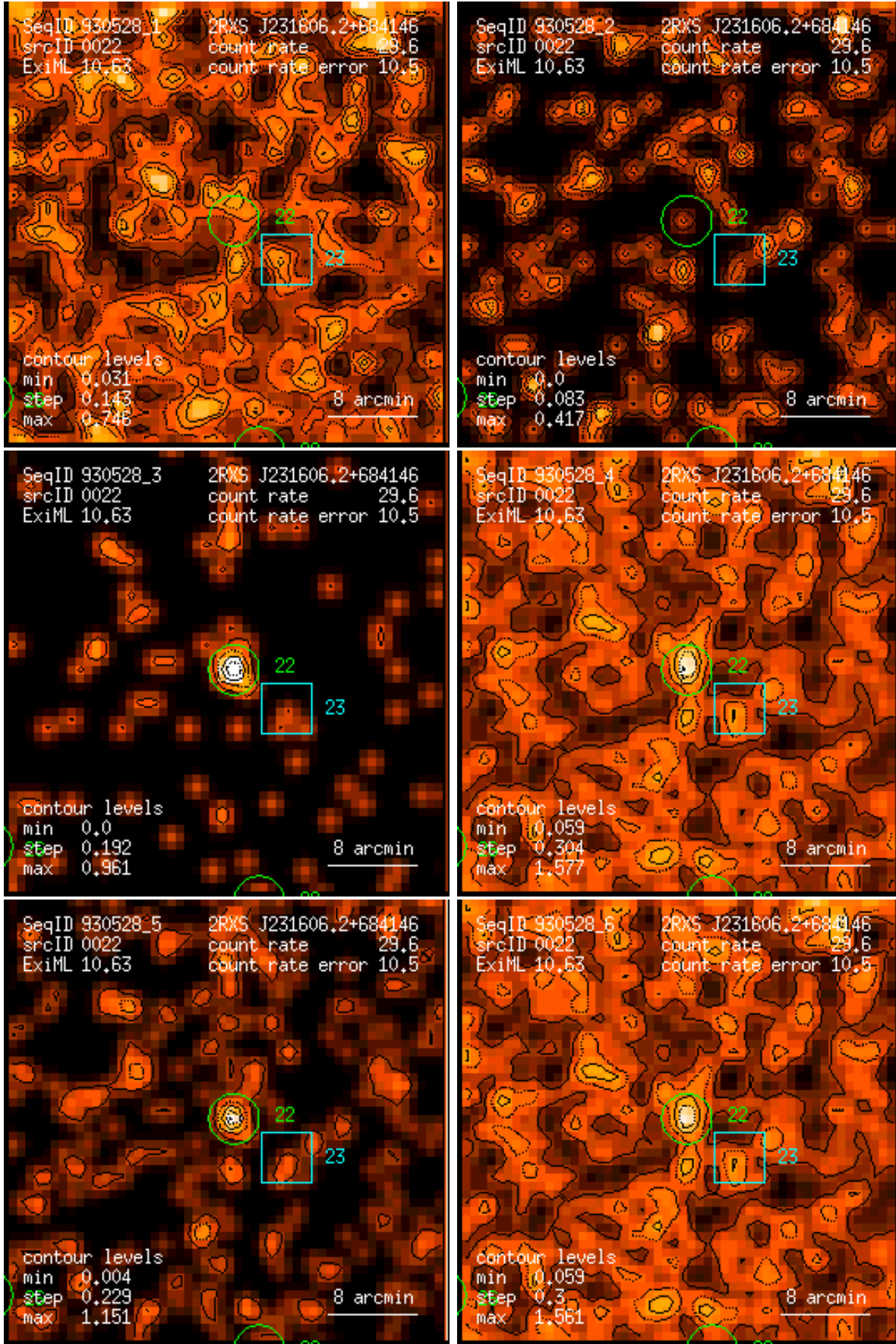
Figure 22: RASS 930528: detection 0022: band rate images, Gaussian filter: (1) PSPC channels 11 – 41, (2) 52 – 90, (3) 91 – 201, (4) 11 – 235, (5) 52 – 201, (6) 11 – 201. Broad band rates in counts/ks. Band rate contour levels in counts/ks/arcmin 2 .
