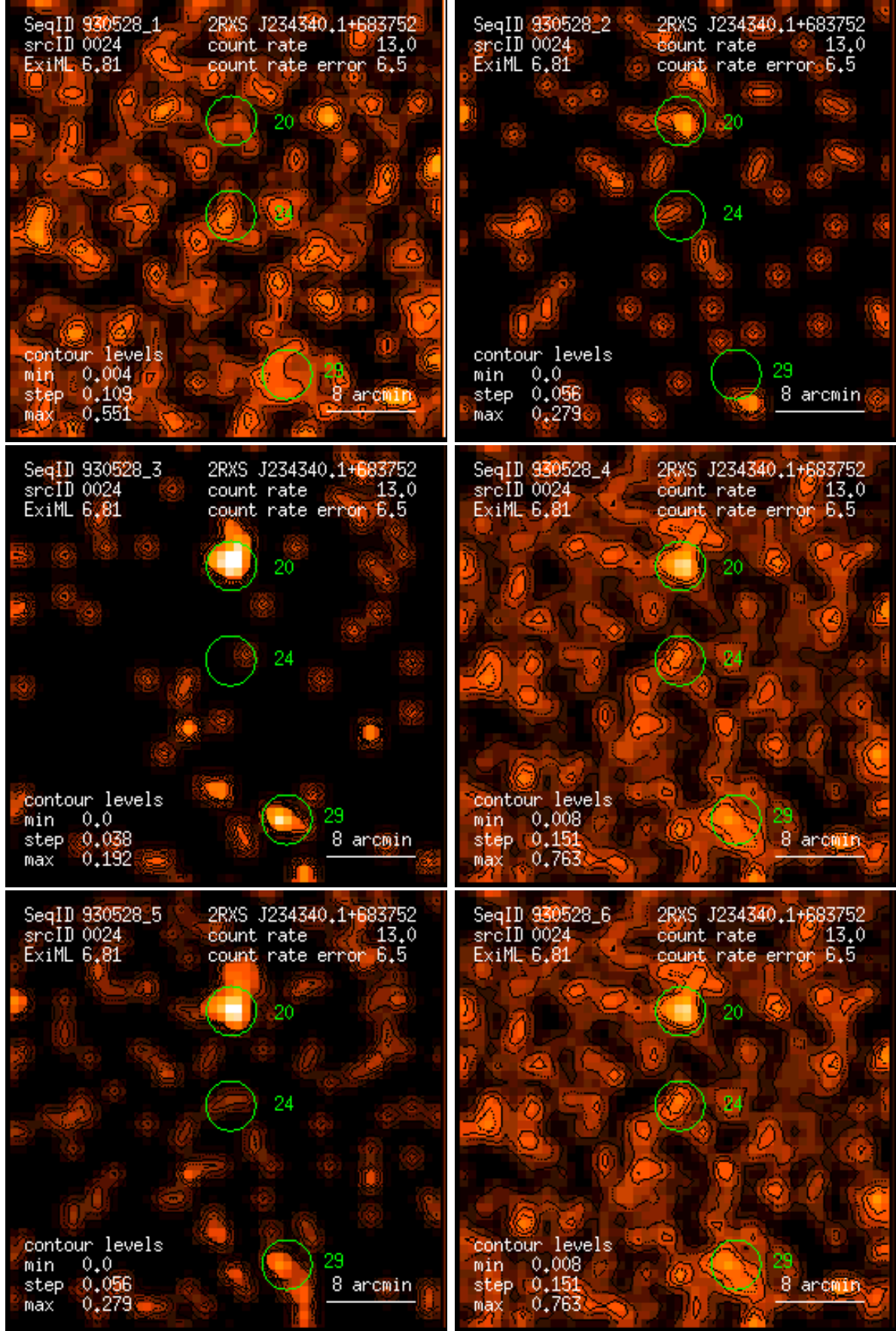
Figure 24: RASS 930528: detection 0024: band rate images, Gaussian filter: (1) PSPC channels 11 – 41, (2) 52 – 90, (3) 91 – 201, (4) 11 – 235, (5) 52 – 201, (6) 11 – 201. Broad band rates in counts/ks. Band rate contour levels in counts/ks/arcmin 2 .
