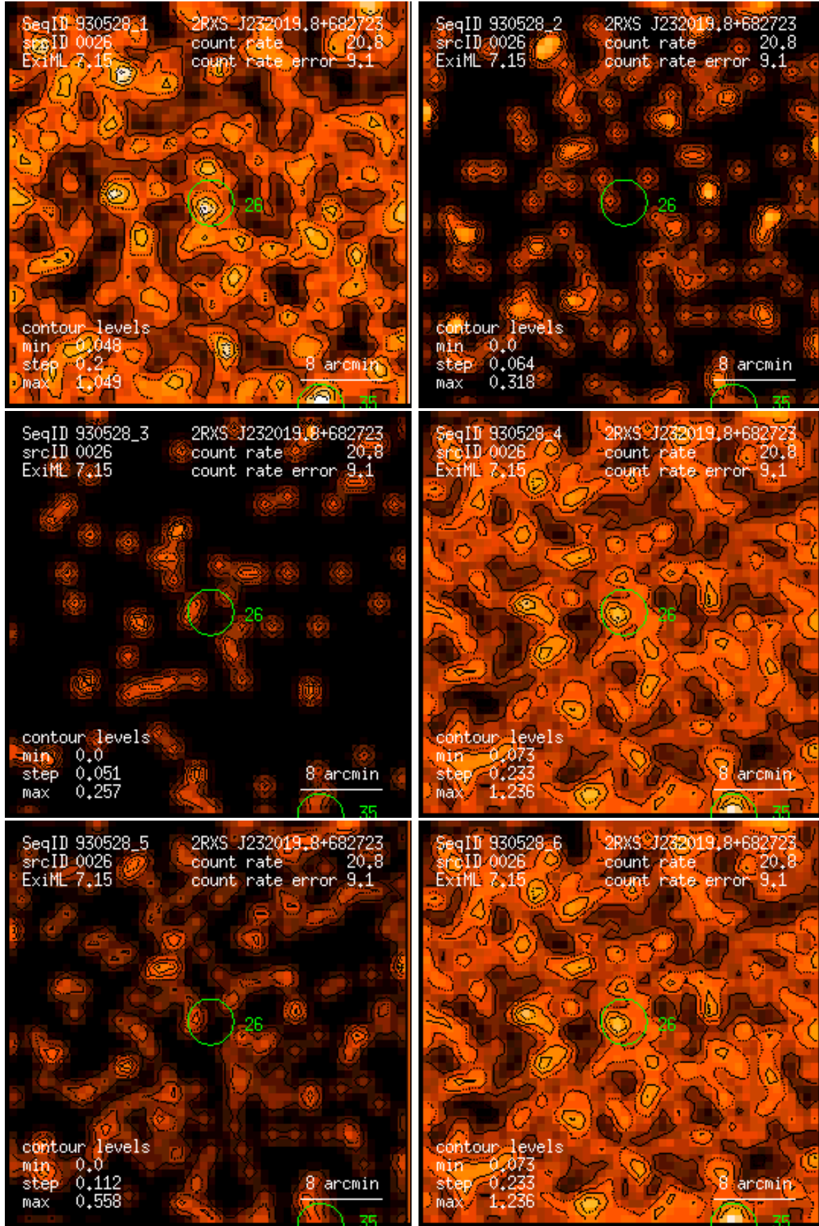
Figure 26: RASS 930528: detection 0026: band rate images, Gaussian filter: (1) PSPC channels 11 – 41, (2) 52 – 90, (3) 91 – 201, (4) 11 – 235, (5) 52 – 201, (6) 11 – 201. Broad band rates in counts/ks. Band rate contour levels in counts/ks/arcmin 2 .
