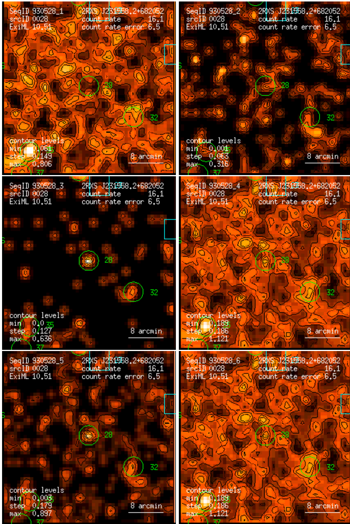
Figure 28: RASS 930528: detection 0028: band rate images, Gaussian filter: (1) PSPC channels 11 – 41, (2) 52 – 90, (3) 91 – 201, (4) 11 – 235, (5) 52 – 201, (6) 11 – 201. Broad band rates in counts/ks. Band rate contour levels in counts/ks/arcmin 2 .
