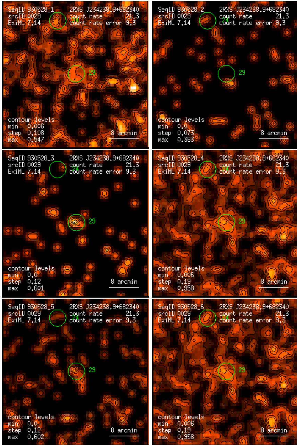
Figure 29: RASS 930528: detection 0029: band rate images, Gaussian filter: (1) PSPC channels 11 – 41, (2) 52 – 90, (3) 91 – 201, (4) 11 – 235, (5) 52 – 201, (6) 11 – 201. Broad band rates in counts/ks. Band rate contour levels in counts/ks/arcmin 2 .
