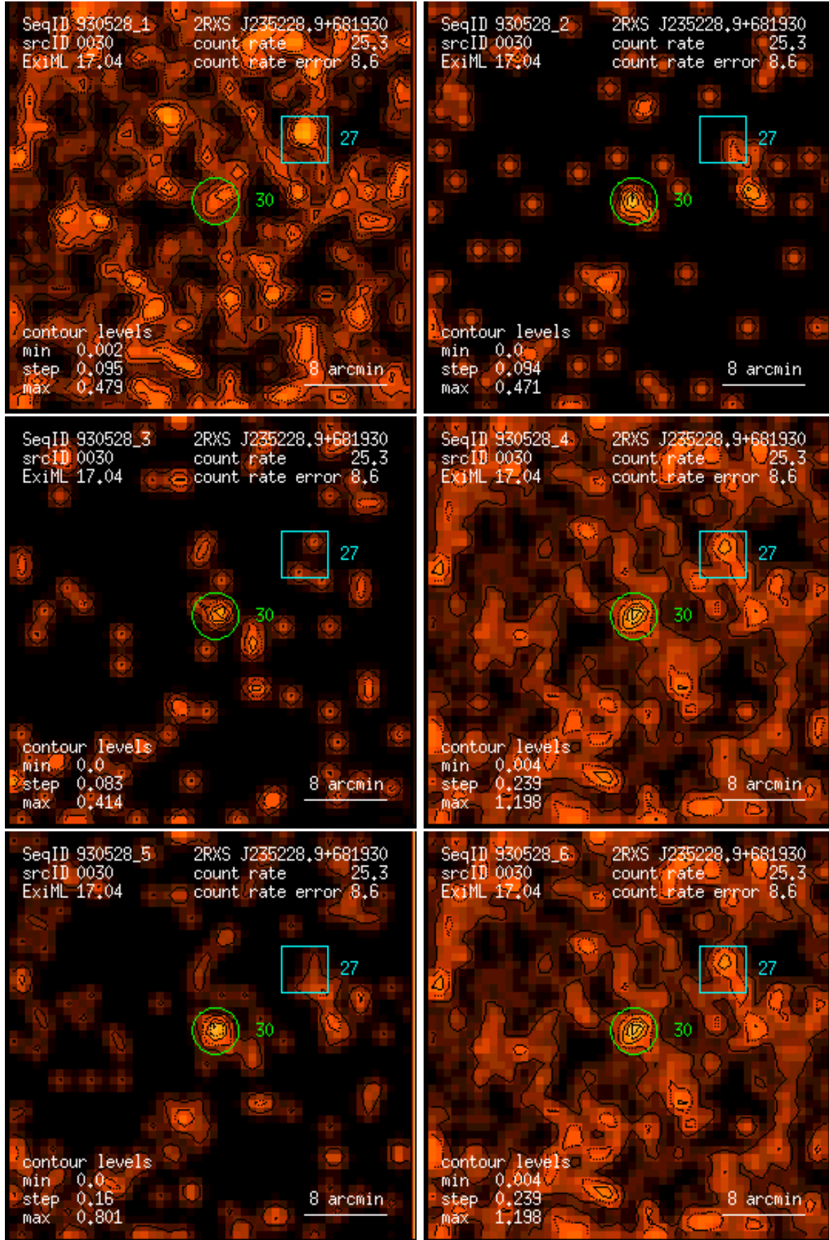
Figure 30: RASS 930528: detection 0030: band rate images, Gaussian filter: (1) PSPC channels 11 – 41, (2) 52 – 90, (3) 91 – 201, (4) 11 – 235, (5) 52 – 201, (6) 11 – 201. Broad band rates in counts/ks. Band rate contour levels in counts/ks/arcmin 2 .
