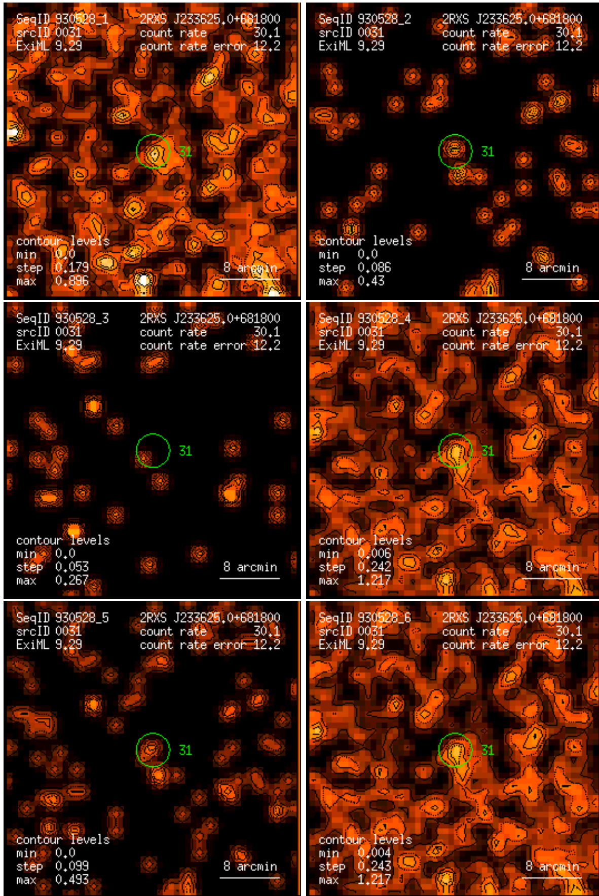
Figure 31: RASS 930528: detection 0031: band rate images, Gaussian filter: (1) PSPC channels 11 – 41, (2) 52 – 90, (3) 91 – 201, (4) 11 – 235, (5) 52 – 201, (6) 11 – 201. Broad band rates in counts/ks. Band rate contour levels in counts/ks/arcmin 2 .
