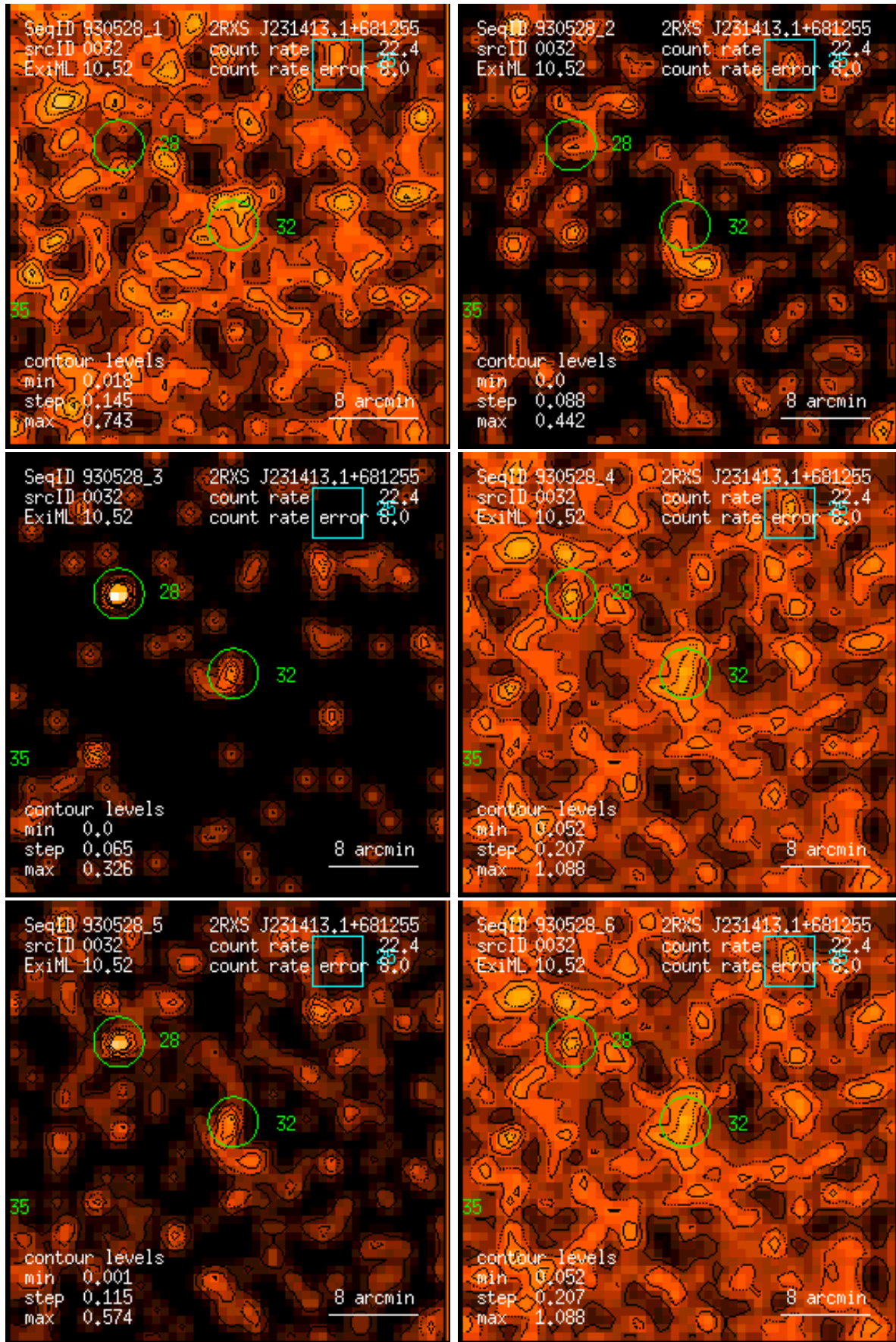
Figure 32: RASS 930528: detection 0032: band rate images, Gaussian filter: (1) PSPC channels 11 – 41, (2) 52 – 90, (3) 91 – 201, (4) 11 – 235, (5) 52 – 201, (6) 11 – 201. Broad band rates in counts/ks. Band rate contour levels in counts/ks/arcmin 2 .
