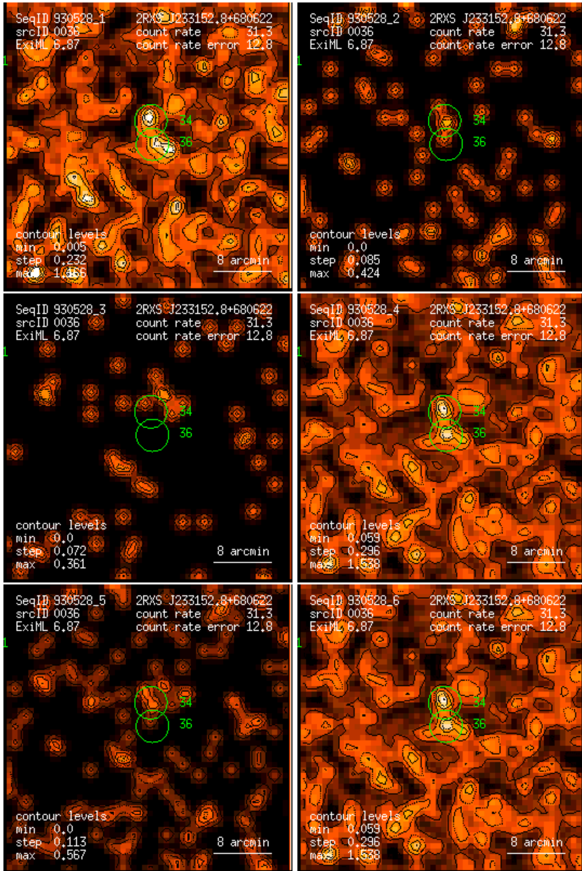
Figure 36: RASS 930528: detection 0036: band rate images, Gaussian filter: (1) PSPC channels 11 – 41, (2) 52 – 90, (3) 91 – 201, (4) 11 – 235, (5) 52 – 201, (6) 11 – 201. Broad band rates in counts/ks. Band rate contour levels in counts/ks/arcmin 2 .
