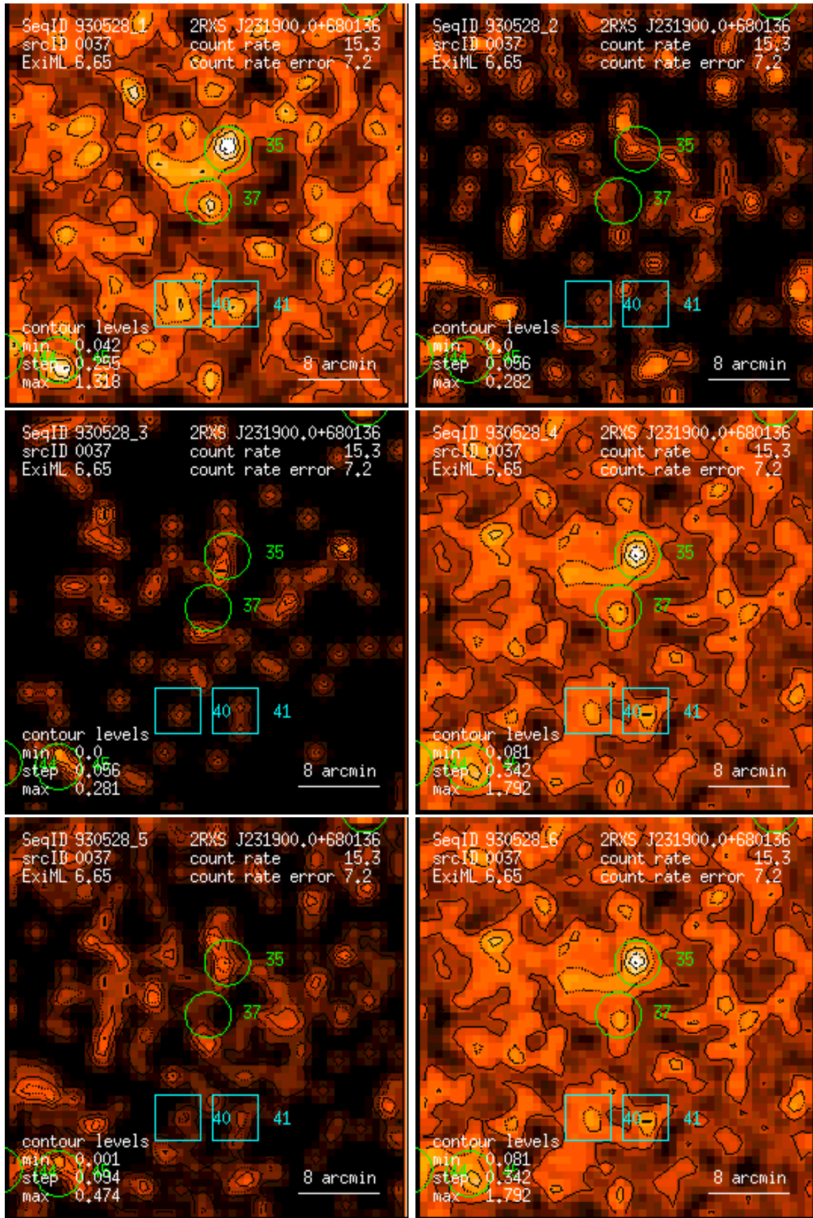
Figure 37: RASS 930528: detection 0037: band rate images, Gaussian filter: (1) PSPC channels 11 – 41, (2) 52 – 90, (3) 91 – 201, (4) 11 – 235, (5) 52 – 201, (6) 11 – 201. Broad band rates in counts/ks. Band rate contour levels in counts/ks/arcmin 2 .
