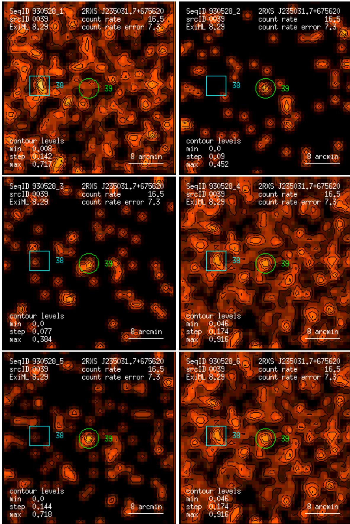
Figure 39: RASS 930528: detection 0039: band rate images, Gaussian filter: (1) PSPC channels 11 – 41, (2) 52 – 90, (3) 91 – 201, (4) 11 – 235, (5) 52 – 201, (6) 11 – 201. Broad band rates in counts/ks. Band rate contour levels in counts/ks/arcmin 2 .
