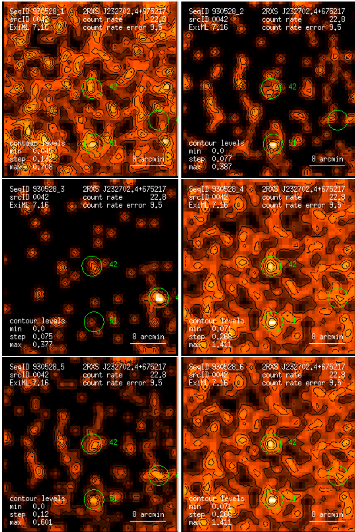
Figure 42: RASS 930528: detection 0042: band rate images, Gaussian filter: (1) PSPC channels 11 – 41, (2) 52 – 90, (3) 91 – 201, (4) 11 – 235, (5) 52 – 201, (6) 11 – 201. Broad band rates in counts/ks. Band rate contour levels in counts/ks/arcmin 2 .
