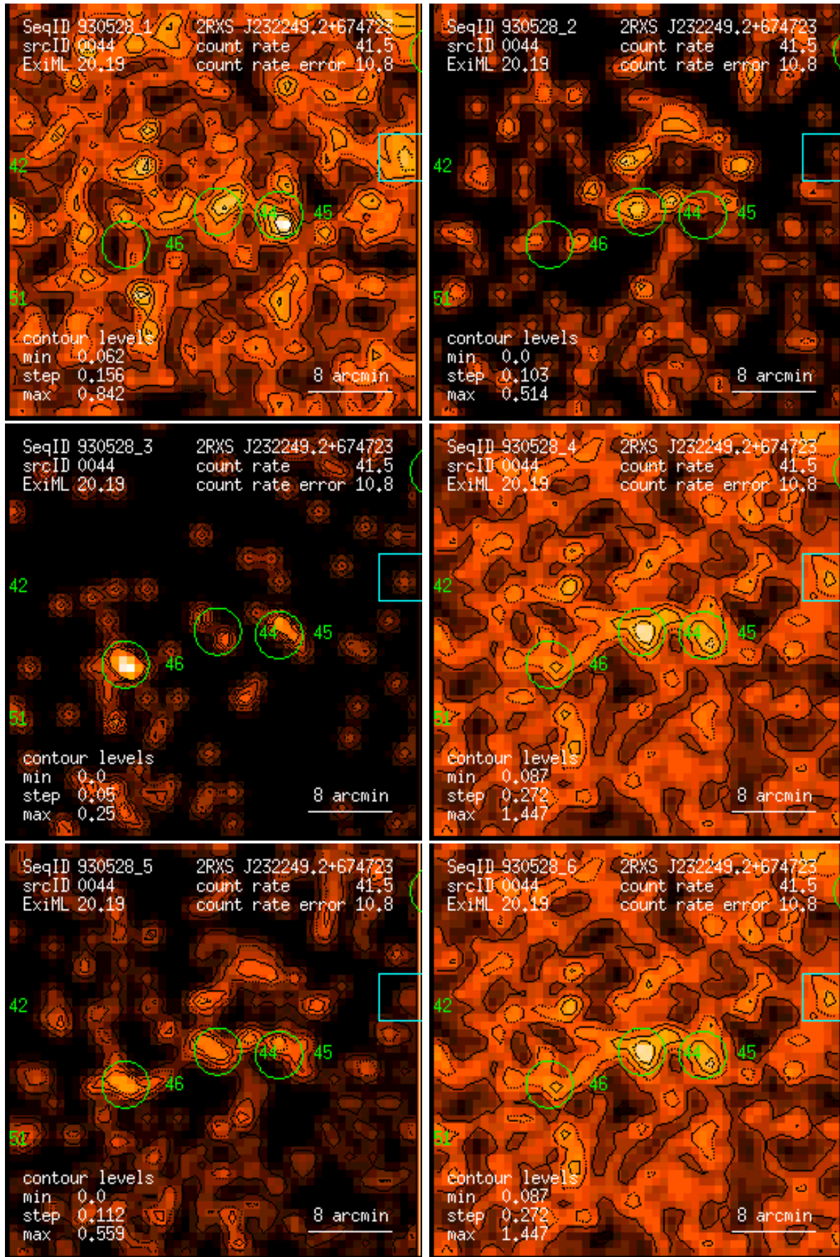
Figure 44: RASS 930528: detection 0044: band rate images, Gaussian filter: (1) PSPC channels 11 – 41, (2) 52 – 90, (3) 91 – 201, (4) 11 – 235, (5) 52 – 201, (6) 11 – 201. Broad band rates in counts/ks. Band rate contour levels in counts/ks/arcmin 2 .
